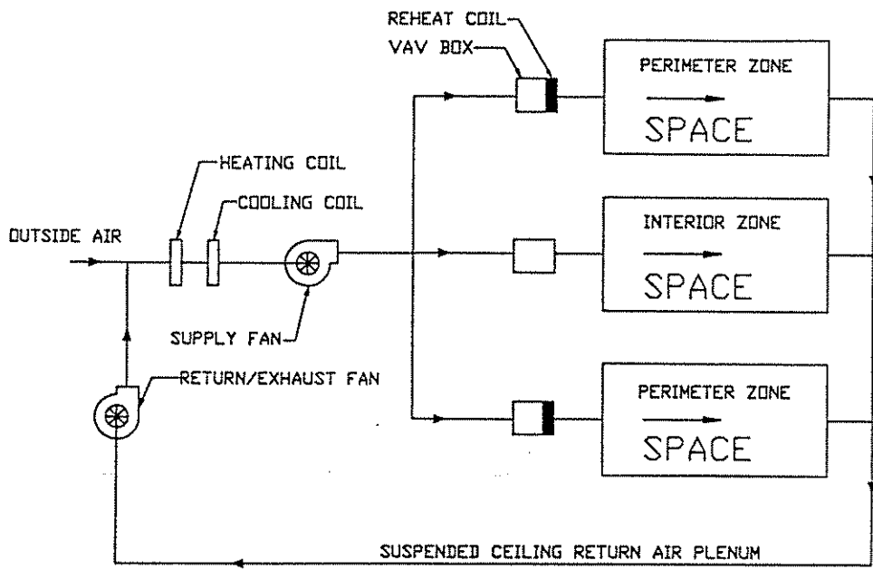
Figure 5.4. Schematic of typical HVAC system used for example building 1.
