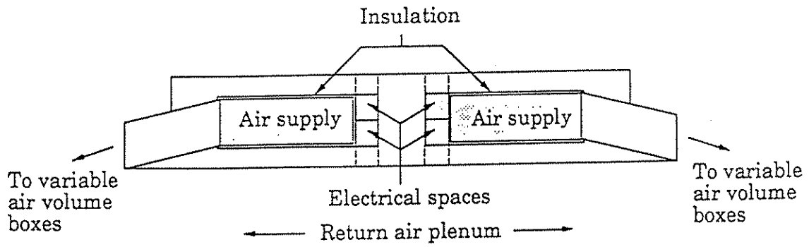
Figure 3.32. Voids in proposed beam can house electrical and HVAC services [adapted from Low 1991].
