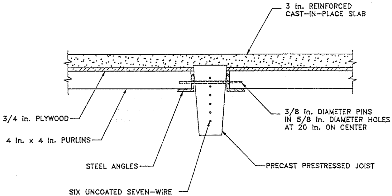
Figure 3.20. Section of precast Keystone joist during erection.
