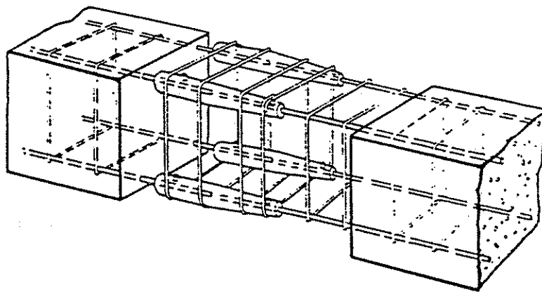
Figure 3.35. Beam-to-beam mechanical splice connection [adapted from Warnes 1991].
