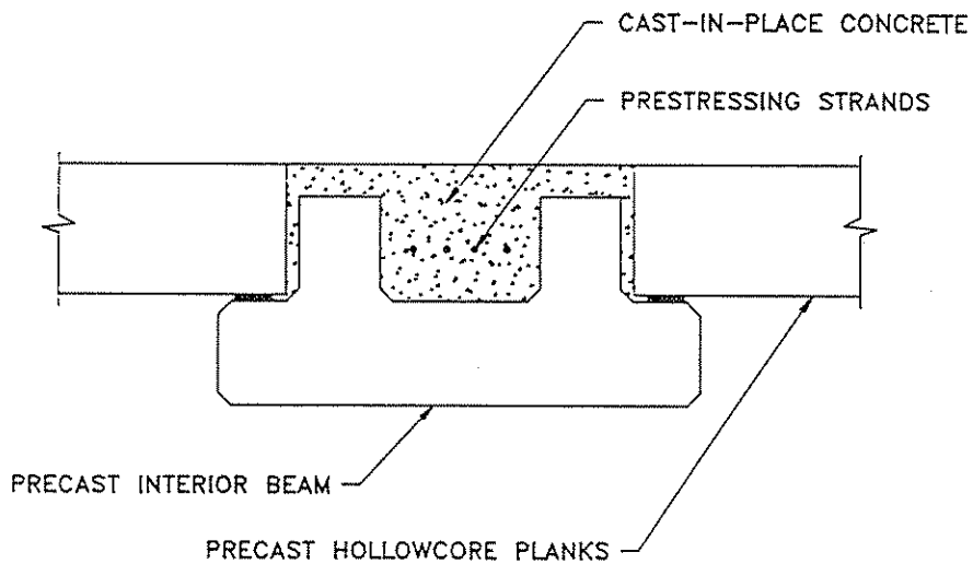
Figure 3.29. Typical spine beam section. Prestressing strands are placed in trough of beam and tensioned.
