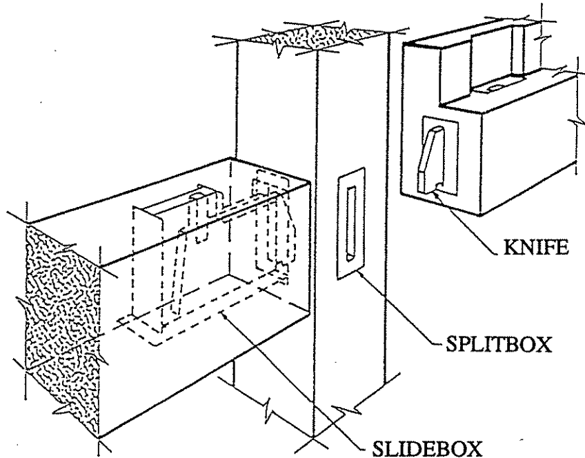
Figure 3.36. The BSF prefabricated beam-to-column shear connection. The steel knife from the beam is slipped into the column splitbox [adapted from Østspenn Holding A/S 1991].
