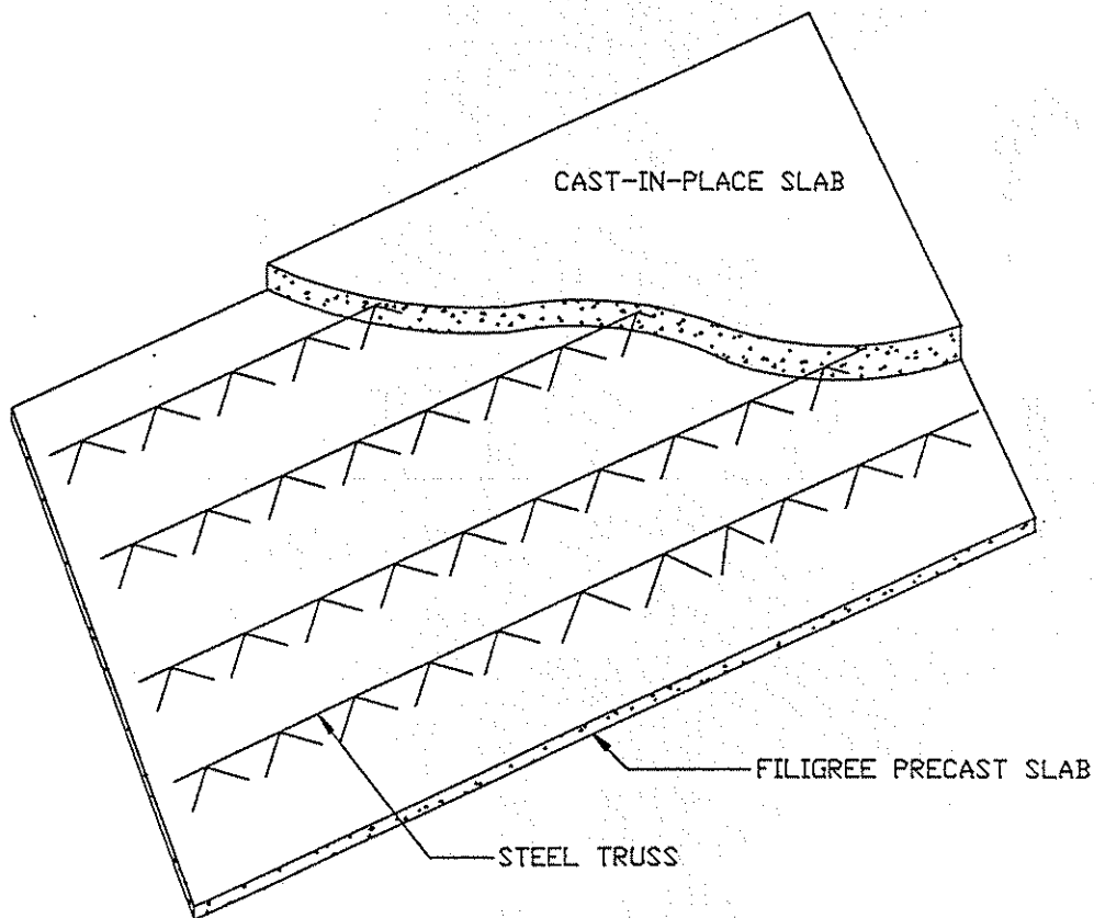
Figure 3.12 Precast slab with light steel truss.
