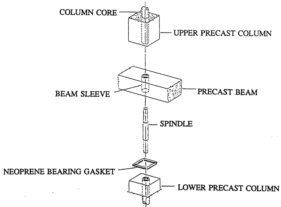
Figure 3.9. Detail showing column-to-beam connection [adapted from Flexicore Systems 1992].
