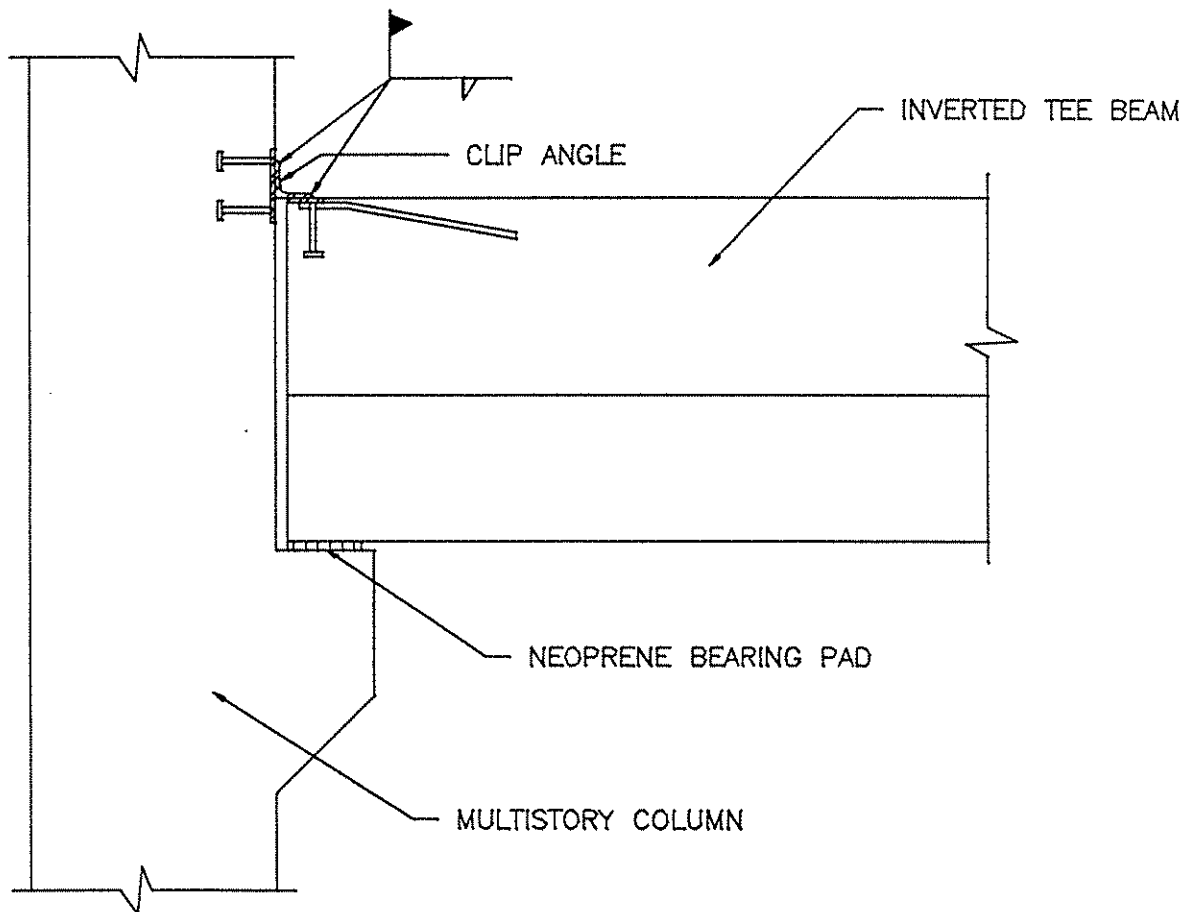
Figure 3.1. Typical beam-to-column connection. Steel plates are anchored with studs into the precast beam and column. A steel angle, welded at the toes, forms the simple connection.
