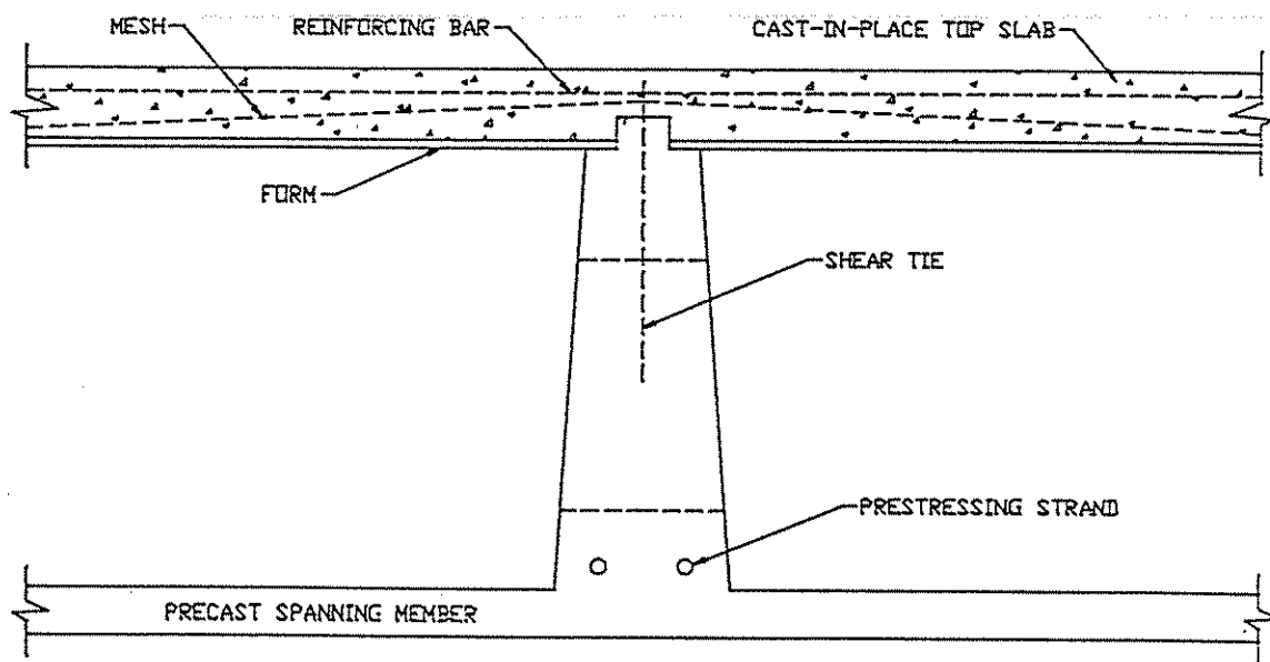
Figure 3.24. Section through Trilposite floor system.
