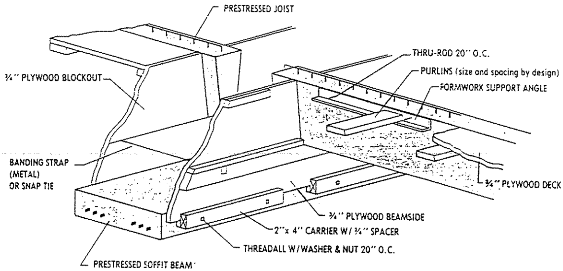
Figure 3.19. Soffit beam assembly for deep beams [adapted from Prestressed Systems Industries].
