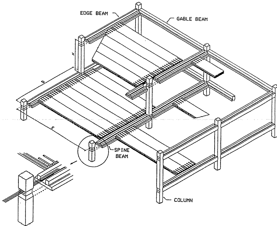
Figure 3.28. Precast structural components. Precast components include spine beams, edge beams and columns. System is post-tensioned from the center of the structure [adapted from Dow Mac 1991].
