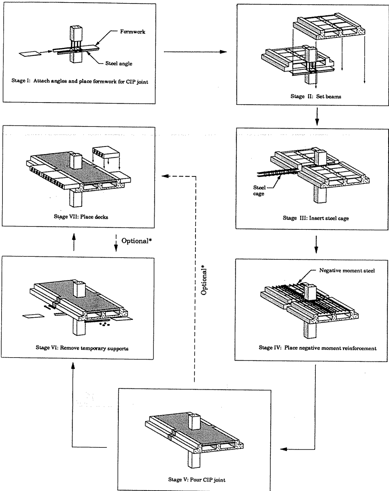
Figure 3.31. VII stage construction sequence [adapted from Low 1991].
