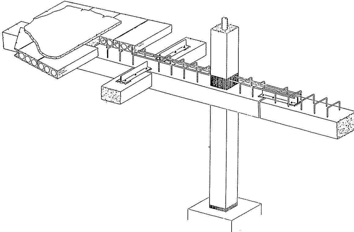
Figure 3.8. Dyna-frame structural components [adapted from Flexicore Systems 1992].
