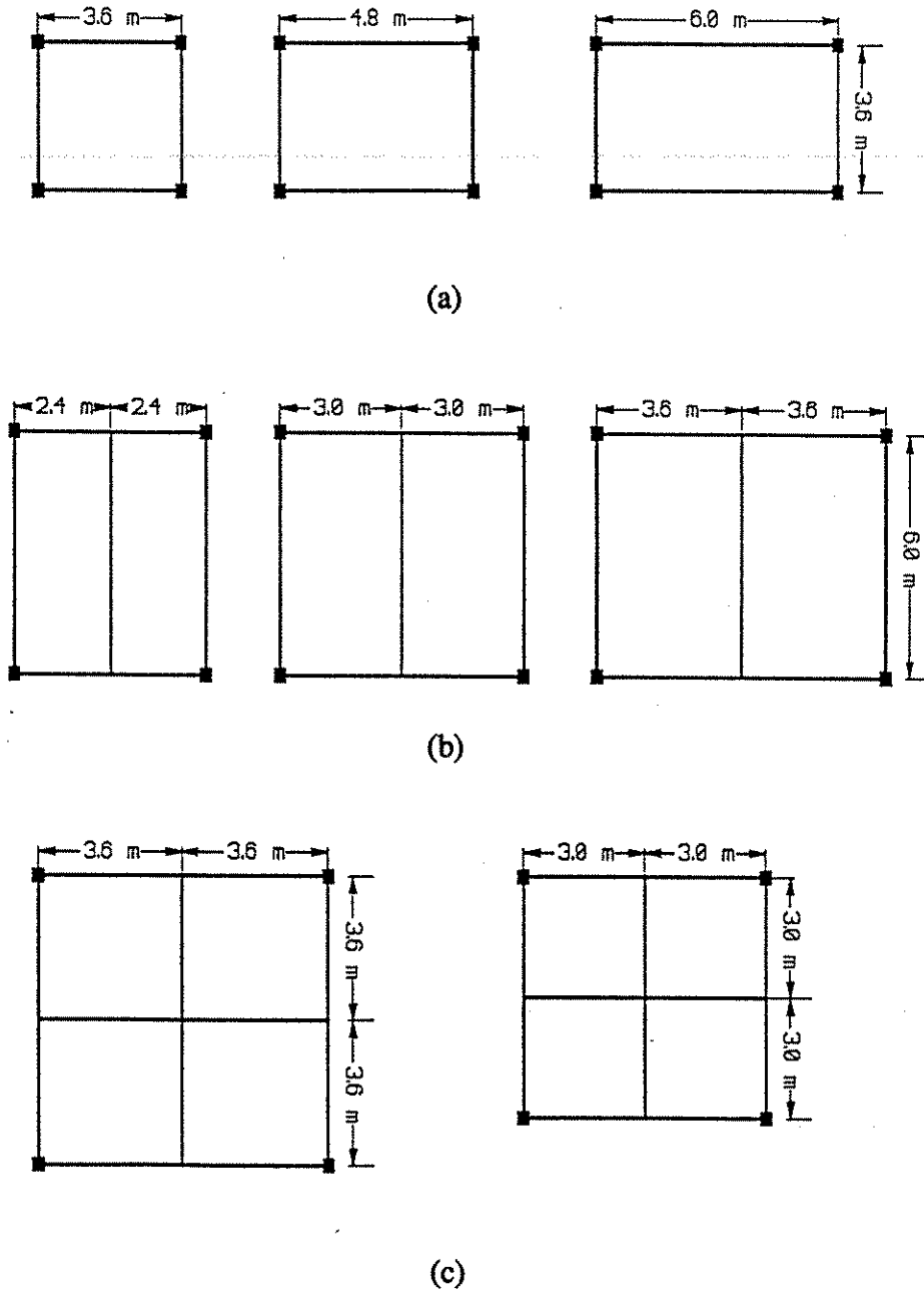
Figure 3.15. Modular composition possibilities for the IMS system: a) Single-unit systems 3.6 x 3.6 m, 4.8 x 3.6 m, or 6.0 x 3.6 m; b) Two-unit systems 2.4 x 6.0 m, 3.0 x 6.0 m, or 3.6 x 6.0 m; c) Four-unit systems 3.6 x 3.6 m, or 3.0 x 3.0 m.
