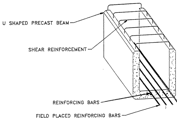
Figure 3.14. U shaped precast shell beam.
