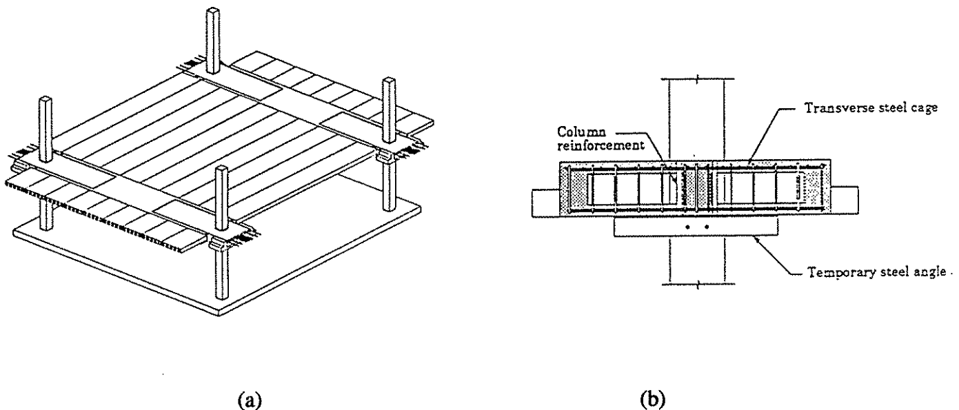
Figure 3.30. Proposed structural system [adapted from Low 1991]: a) Overview of system; b) Beam-to-column detail.
