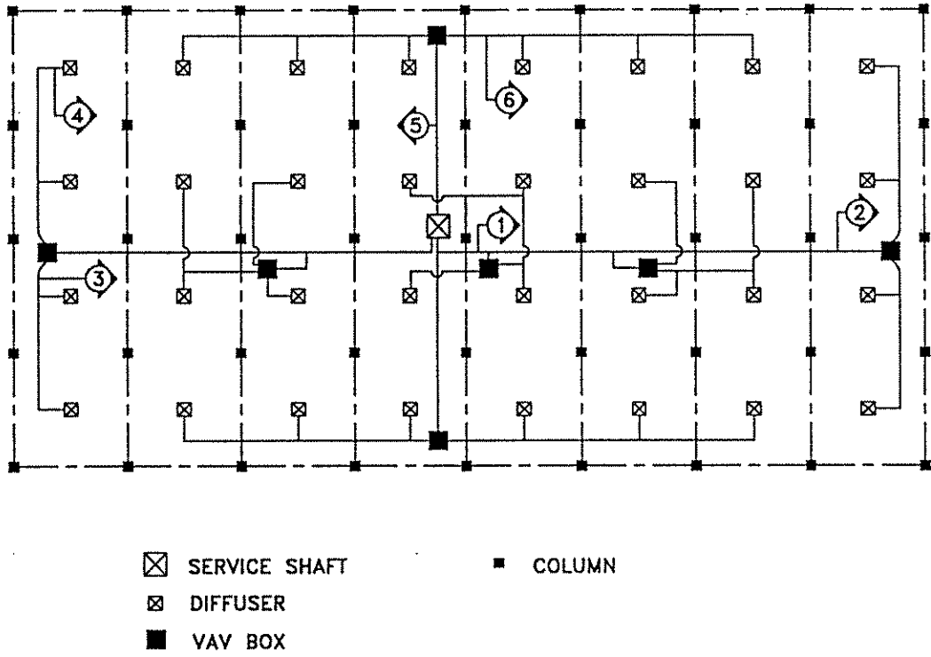
Figure 5.5. HVAC layout, example building 1.
