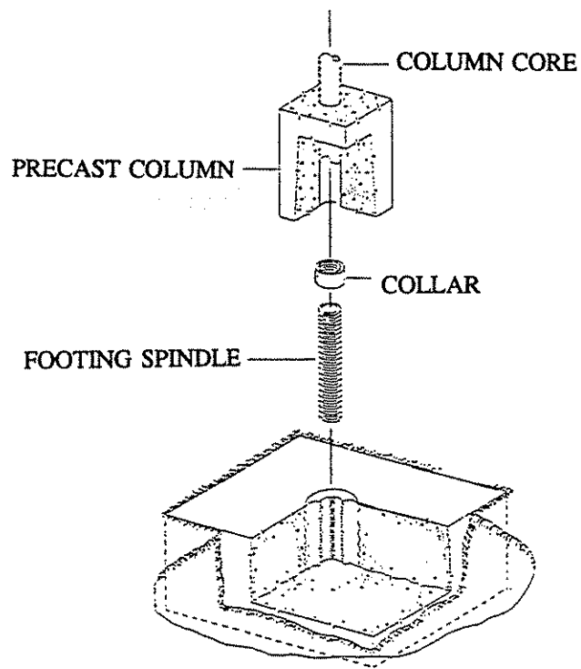
Figure 3.10. Detail showing column footing [adapted from Flexicore Systems 1992].
