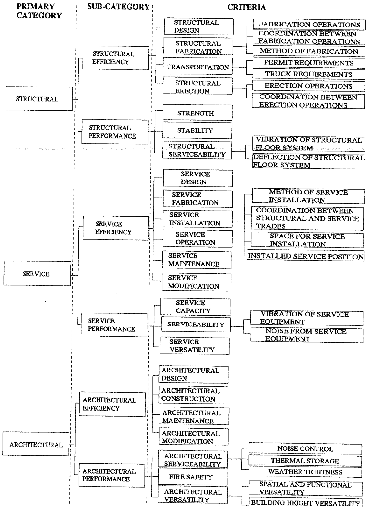
Figure 4.1. Structural, Service, and Architectural criteria.
