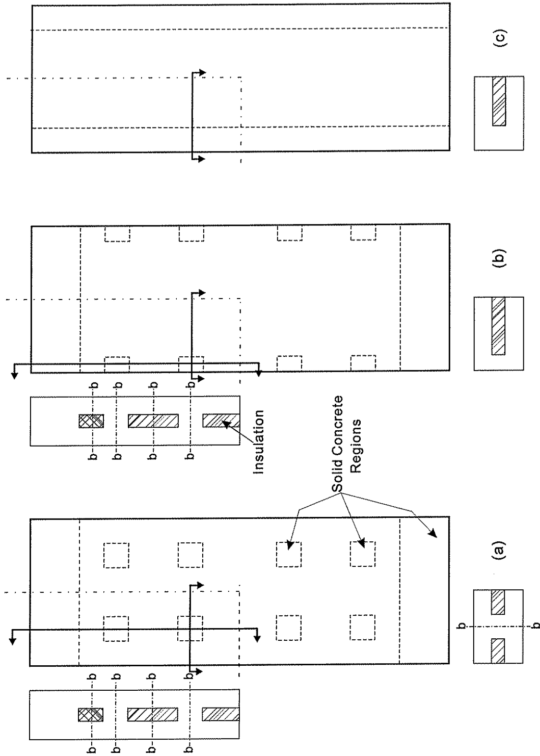
Figure 4.2 Defining a characteristic section from three typical precast concrete sandwich wall panels.
