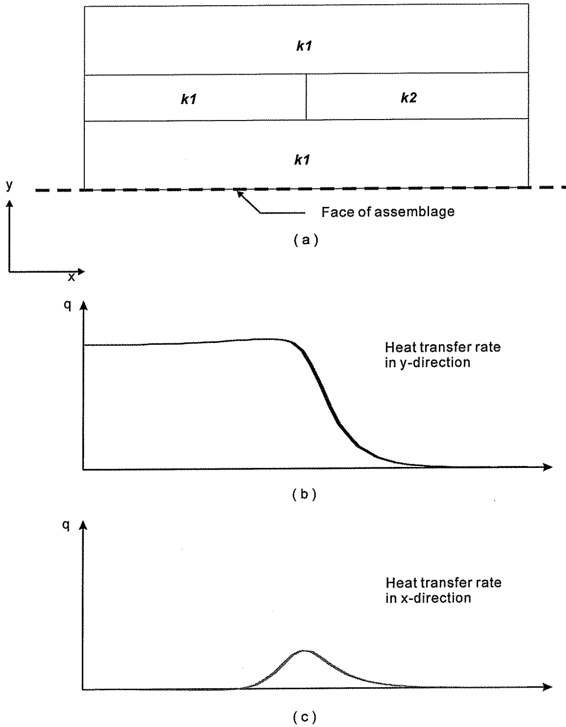
Figure 3.7 Results from the finite element method analysis: (a) assemblage of material; (b) heat transfer rate in y -direction at face; (c) heat transfer rate in x -direction at face.
