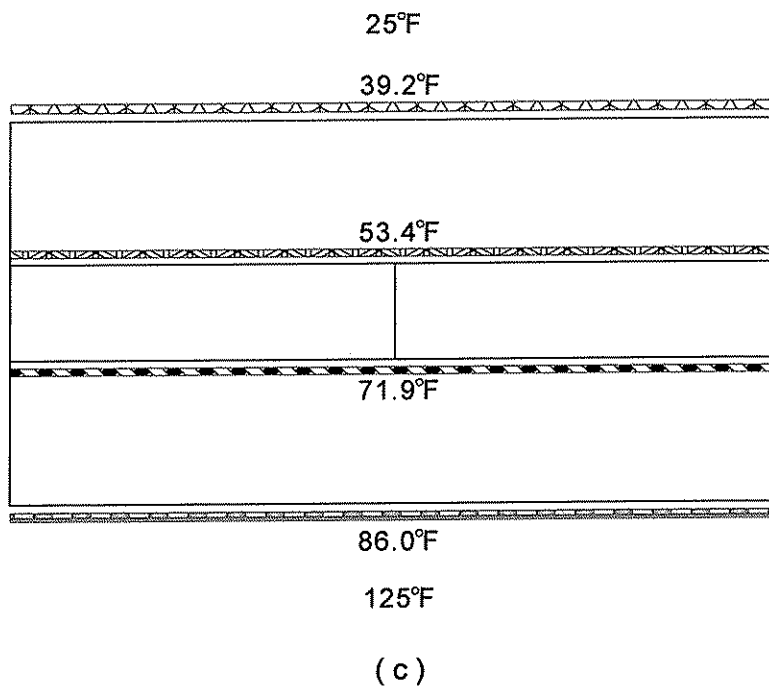
Figure 3.5 Summary of results of isothermal plane calculations: (a) thermal resistance; (b) heat flux; (c) temperature distribution.
