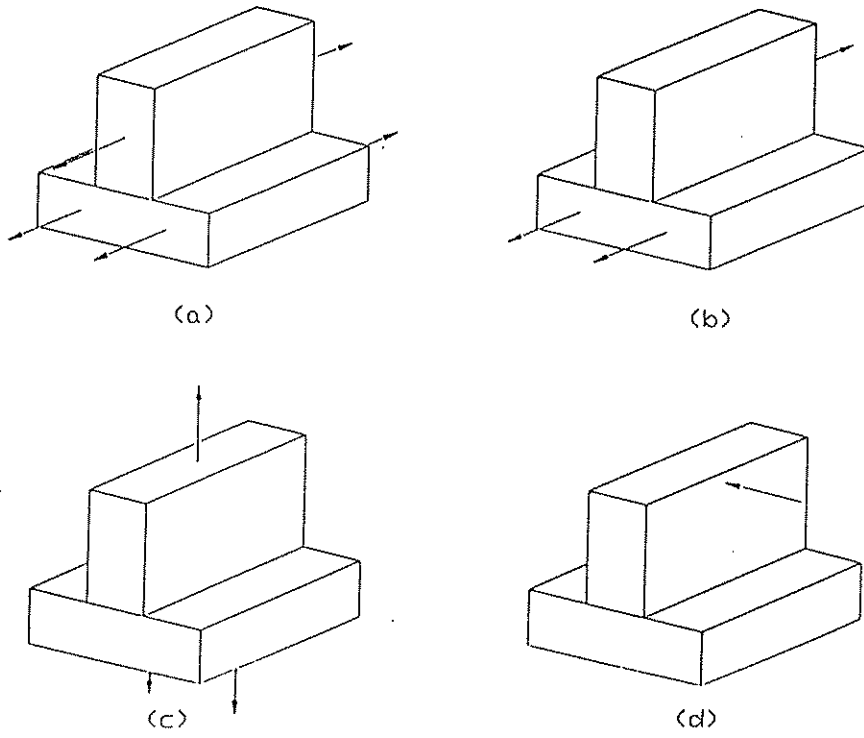
Figure 2-4 Tee Joints and Loadings
