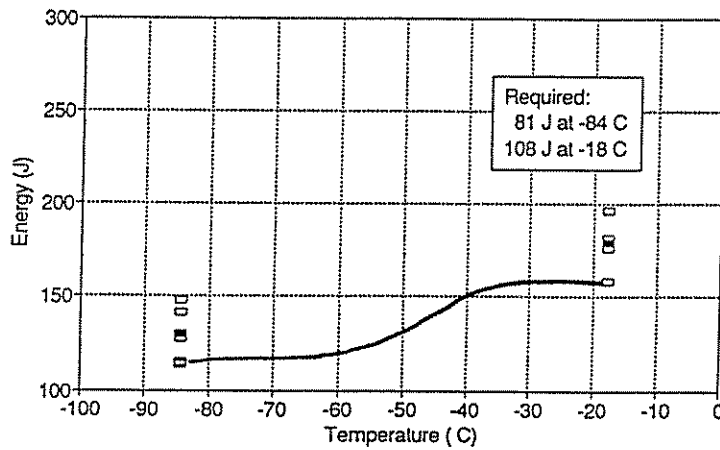
Figure 3-1 Charpy Toughness Data for HSLA-100 Plates in First Series of Tests.
