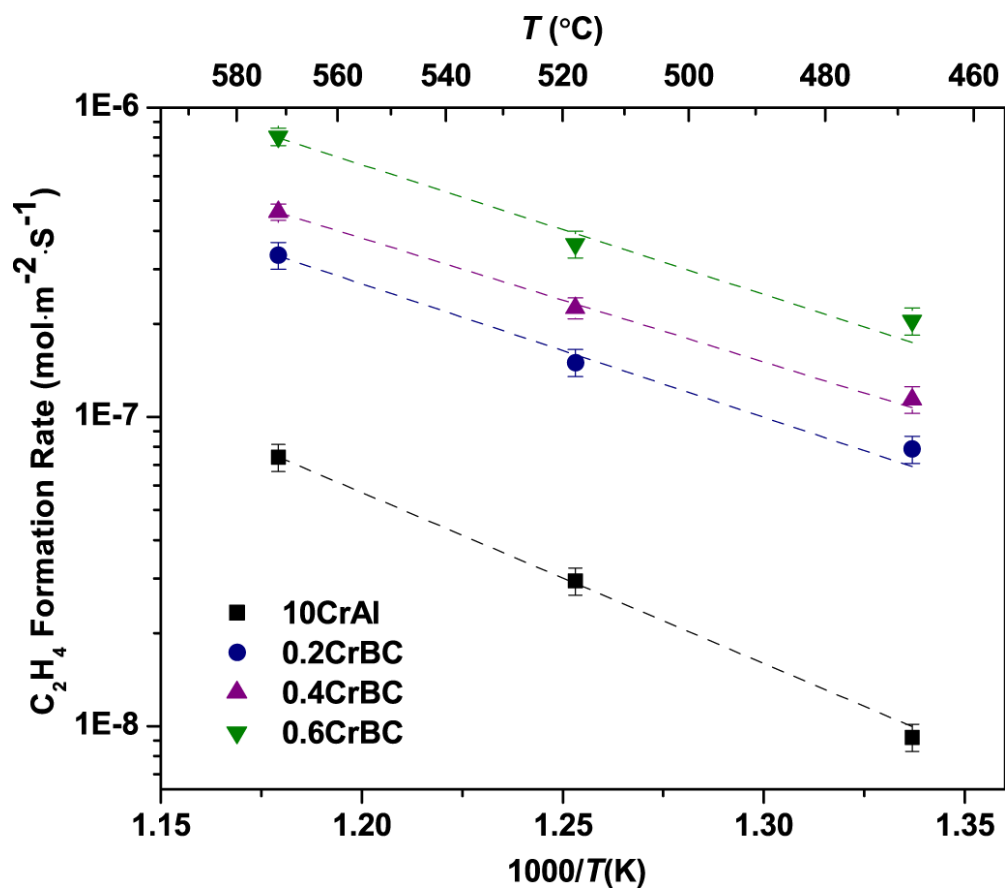
Figure 4.7 Arrhenius plot of ethylene formation rate over Cr/BC and 10CrAl at residence time of 0.13 sec.
