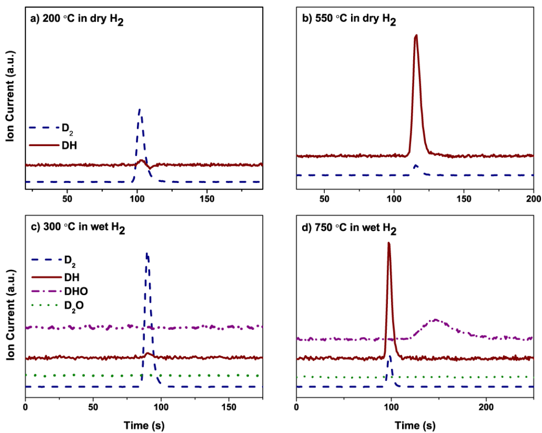
Figure 2.3 DH formation and D 2 consumption in a single pulse (100 \mu L, 5% D 2 ) over BZ in dry H 2 at a) 200 °C and b) 550 °C, DH and DHO formation and D 2 consumption in wet H 2 at c) 300 °C and d) 750 °C
