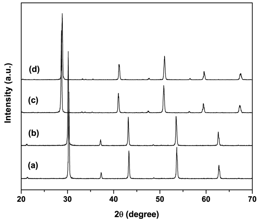
Figure 4.1 X-ray diffraction patterns of (a) BZ, (b) 0.6Cr/BZ, (c) BC and (d) 0.6Cr/BC
