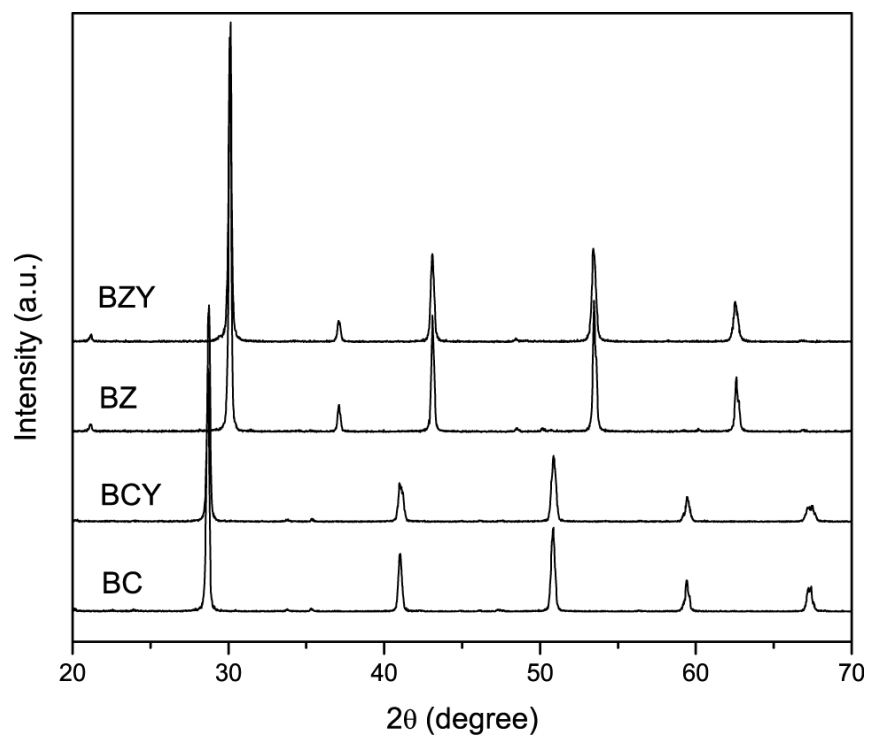
Figure 2.1 X-ray diffraction patterns of BC, BCY, BZ and BZY
