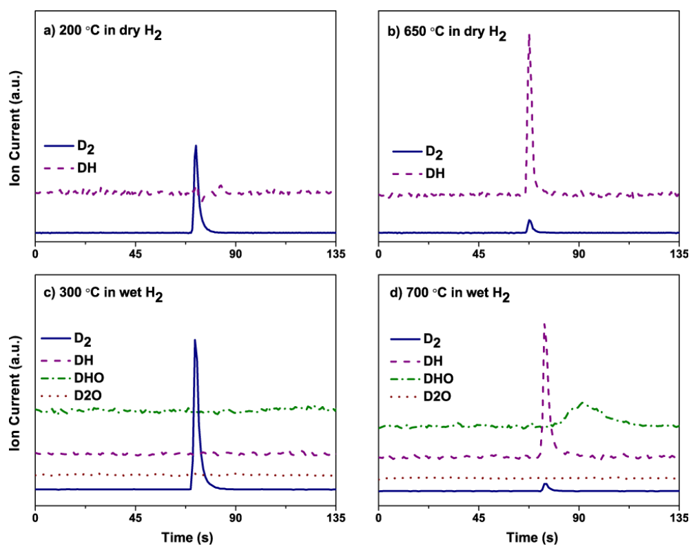
Figure 3.1 DH formation and D 2 consumption in a single pulse (100 μL, 5% D 2 ) over YSZ in dry H 2 at a) 200 °C and b) 650 °C, DH and DHO formation and D 2 consumption in wet H 2 at c) 300 °C and d) 700 °C
