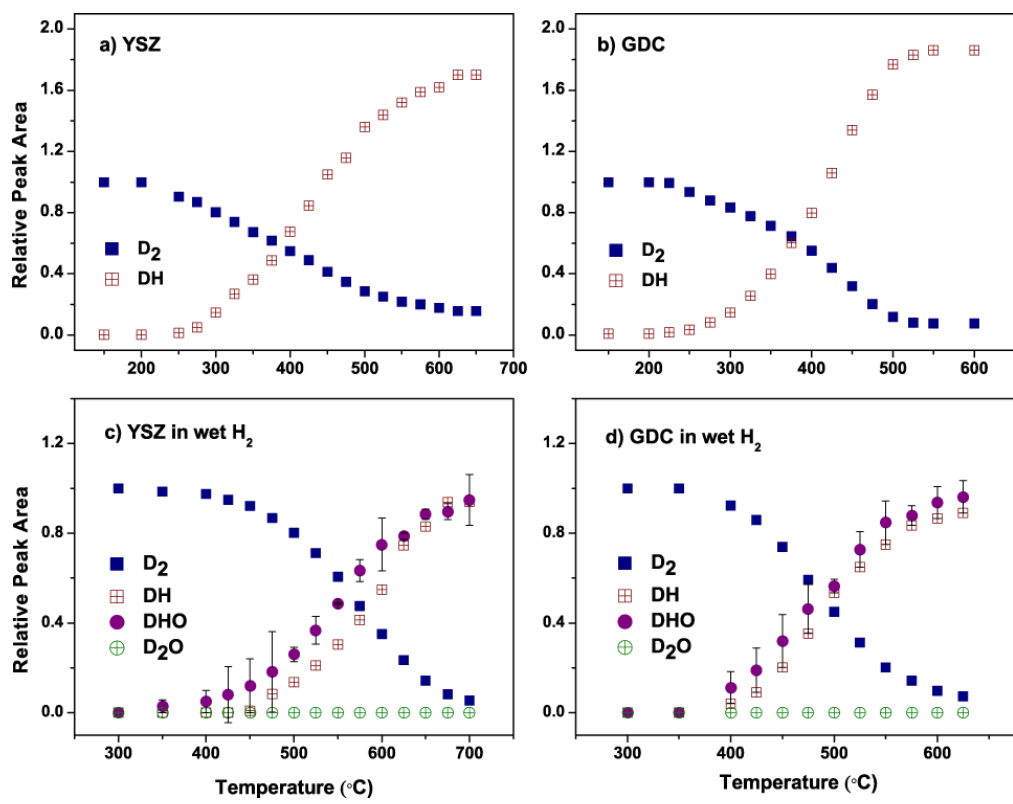
Figure 3.2 Relative peak area of D_2 and DH as a function of temperature for (a) YSZ, (b) GDC in dry H_2 , D_2 , DH and DHO for (c) YSZ, (d) GDC in wet H_2 .
