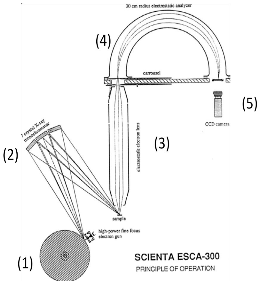
Figure 3.6 Main components of a Scienta ESCA-300 system.
