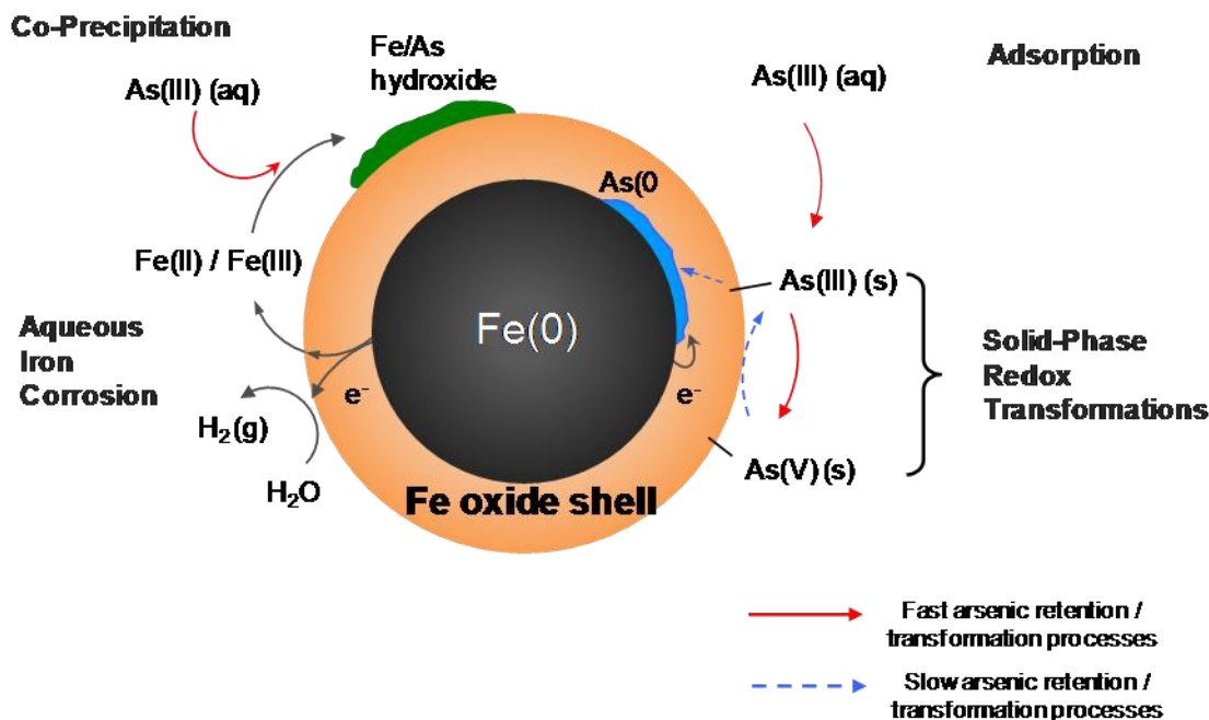
Figure 7.17 Schematic diagram summarizing processes responsible for arsenic removal in As(III)-nZVI system in anoxic conditions. The relative scale of the core and shell components of nZVI are for illustration only and do not reflect actual dimensions. As(III) may be taken up from the aqueous phase by adsorption or co-precipitation. The solid-bound As(III) is oxidized rapidly at the oxide surface, and the As(V) formed may be reverted to As(III) at a slower rate. Some As(III) diffuses towards Fe(0) core and is reduced to elemental arsenic (As(0)) near the oxide/Fe(0) interface.
