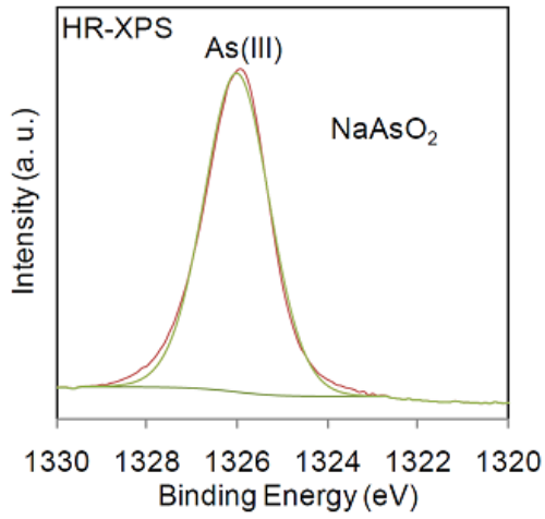
(a) As2p 3/2
