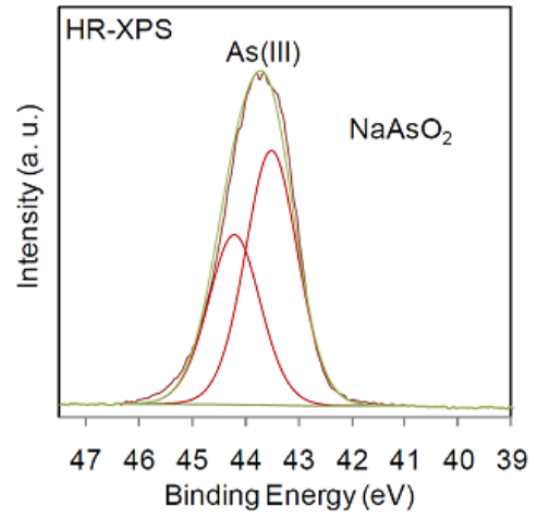
(b) As3d
