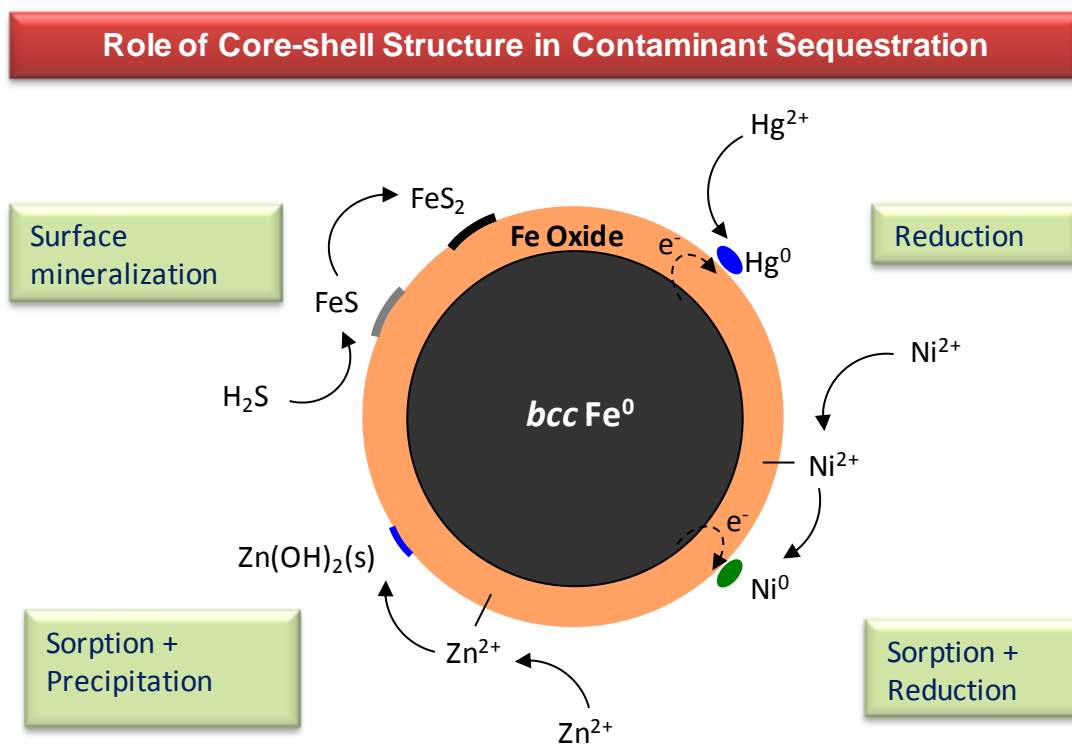
Figure 6.1 The core-shell model of nZVI and schematic representations of the reaction mechanisms for the removal of Hg(II), Ni(II), Zn(II) and H_2S investigated in this study.
