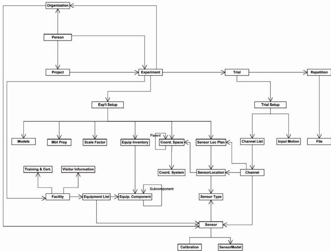
Figure 2.4 NEEScentral Model (NEESit, 2006)
