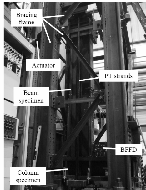
c. Photo of Test Setup
