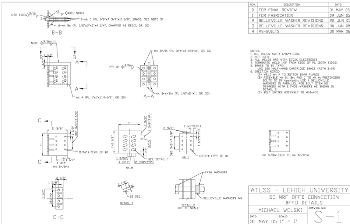
Figure 5.11 Tab S-1 of Setup Drawing File
