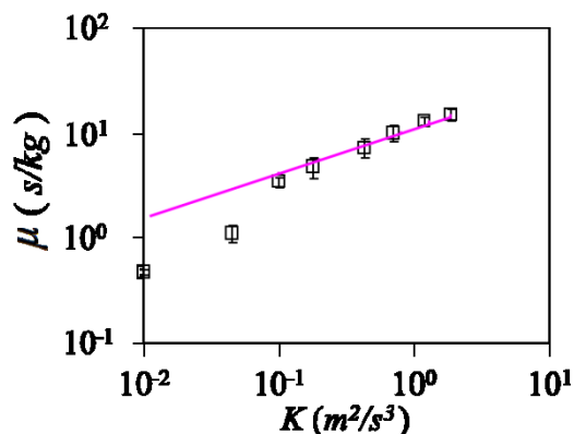
Figure 4.17: The mobility of PDMS grafted glass prism on a PDMS grafted silicon wafer as a function of the power ( K ) of the Gaussian noises but at a constant bias 0.29\text{ mN} . The open squares are the experimental data. The solid line represents the mobilities estimated by dividing the drift velocity (first moment of the PDF given by Eq. 4.6 with A = 0.03 and n = 0.4 ) with the applied bias force ( m\bar{\gamma} ).
