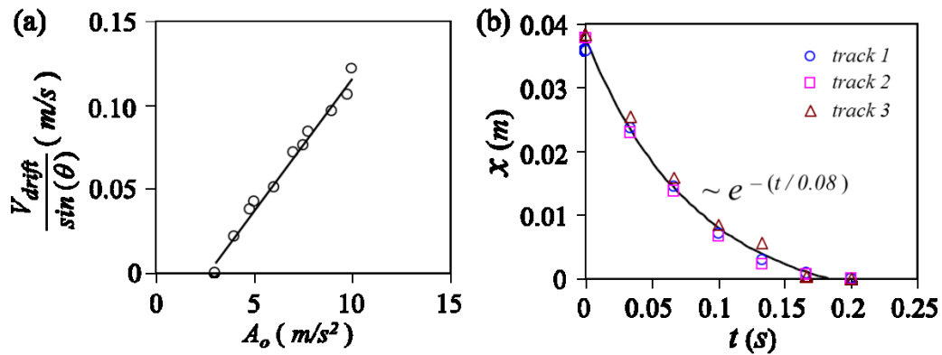
Figure 4.22: (a) Plot of V_{drift}/\sin(\theta) as a function of amplitude of sine wave of 100 Hz for a glass prism on a rough glass support. (b) Plot of displacement (which needs to be traversed before stopping) as a function of time for a glass prism on a horizontal rough glass support when the former is knocked at an edge. Three tracks nicely fall on a single curve having exponential relaxation.
