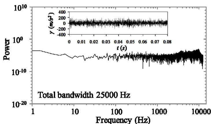
Figure 2.4: A typical trace of the acceleration pulses (inset) corresponding to strength K = 0.16 \text{ m}^2/\text{s}^3 . Corresponding power spectrum taken at a bandwidth of 25kHz.
