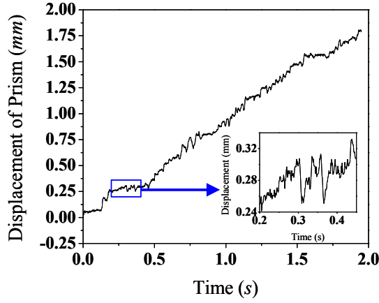
Figure 3.3: Stochastic motion of prism on solid substrate subjected to truncated Cauchy noise of power 0.053 \text{ m}^2/\text{s}^3 .
