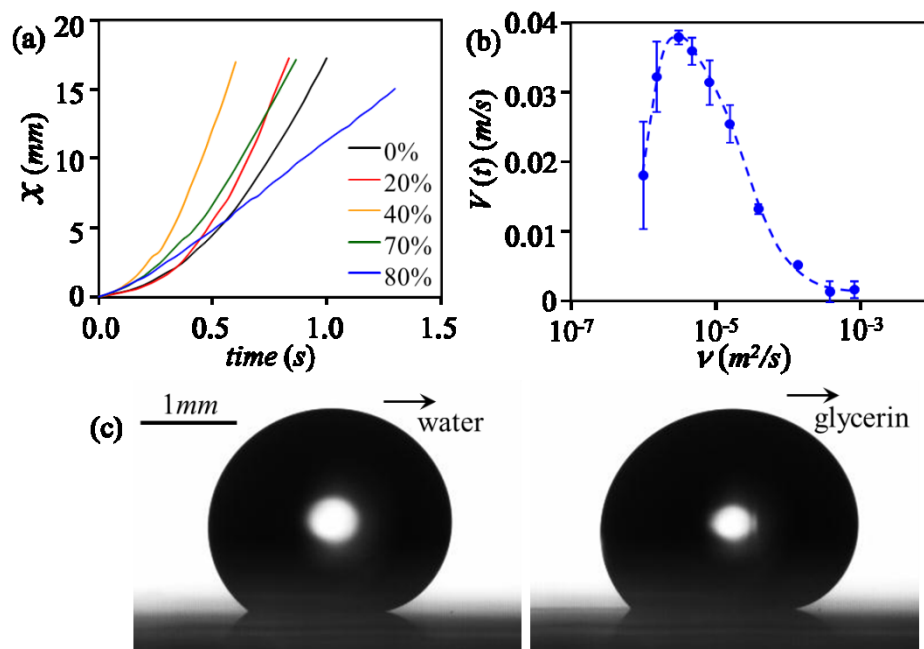
Figure 8.3: (a) Sample trajectories of liquid drops of water and the solutions of glycerin and water on a 10^0 inclined PDMS substrate that had the fibrillar spacing of 50 \mu m . In these trajectories, the initial pause periods are not shown. The compositions of the solutions in terms of the percentage of glycerin in water are stamped inside the figure (b) Drift velocities as measured from the displacement-time trajectories at long time limit are shown in terms of the kinematic viscosity of the glycerin water solutions. (c) Video micrographs of a 10 \mu l drop of water and glycerol slowly moving on a fibrillar PDMS surface of 50 \mu m spacing, inclined by an angle of 10^0 . Advancing and receding contact angles are 160^0 and 139^0 for water and 162^0 and 139^0 for glycerin respectively.
