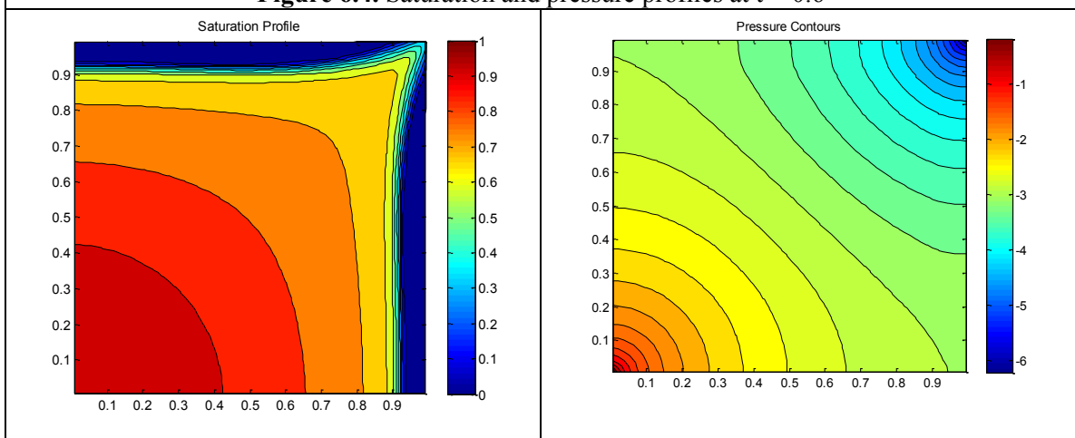
Figure 6.5. Saturation and pressure profiles at t = 0.7
