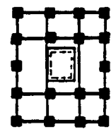
Hat/Belt Trusses & Braced Core
