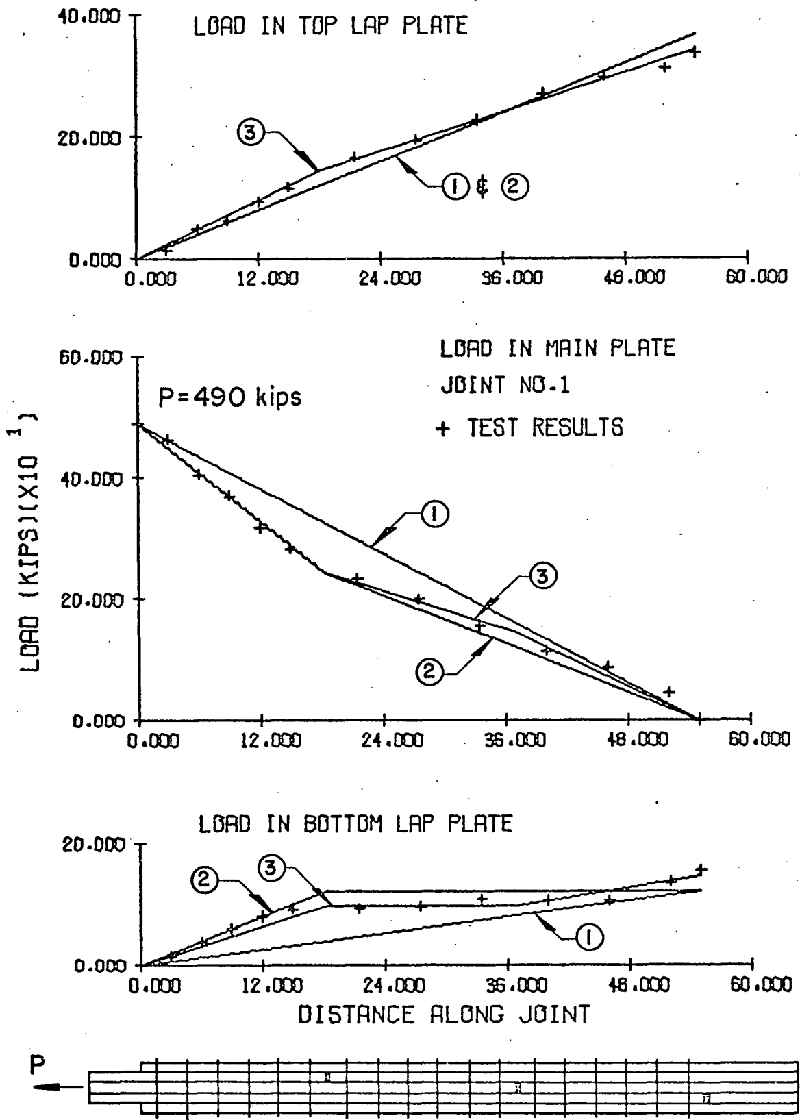
Fig. 12 Comparison of Design Methods with Test Results of Joint 1
