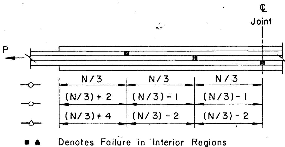
Fig. 4 Effect of Rearranging Fasteners
