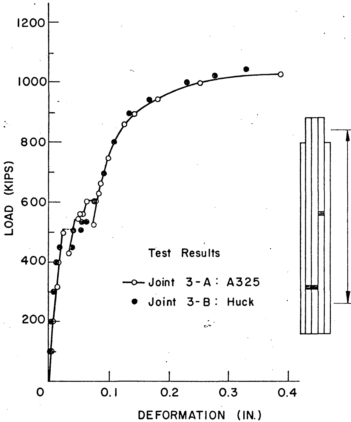
Fig. 7 Comparison of the Load-Deformation Behavior in A325 and Huck-Bolted Joints
