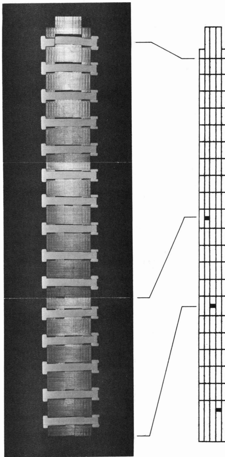
Fig. 9 Sawed Section of Joint 8 After Failure
