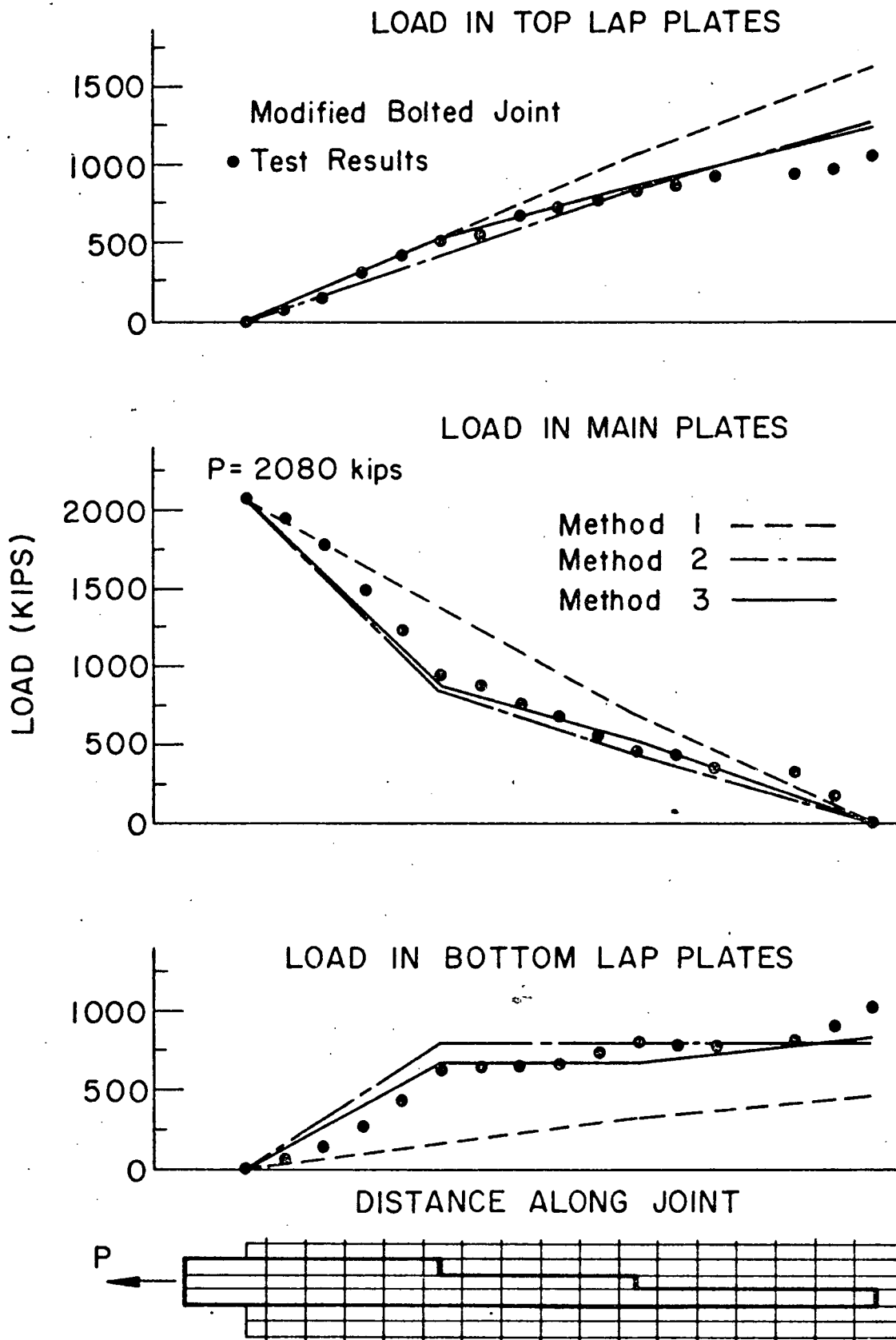
Fig. 13 Comparison of Design Methods with the Experimental Load Partition in the Modified Bolted Joint
