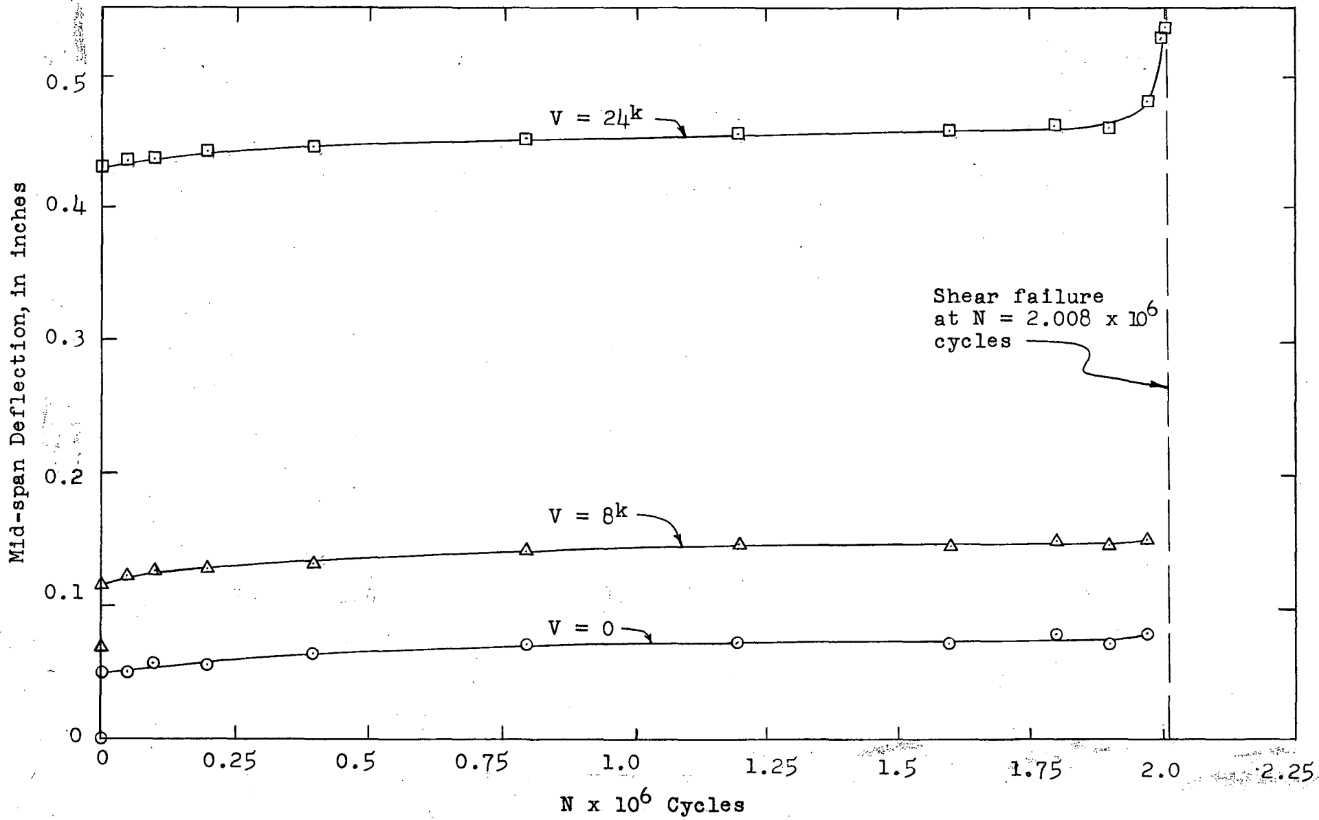
Figure 9. Deflection - N curve for E.11
