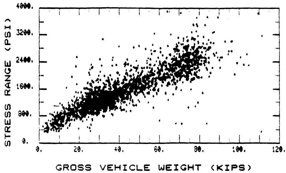
Fig. 6 Stress Range vs GWW - Bottom Flange - Midspan of First Interior Girder of Bridge 1
