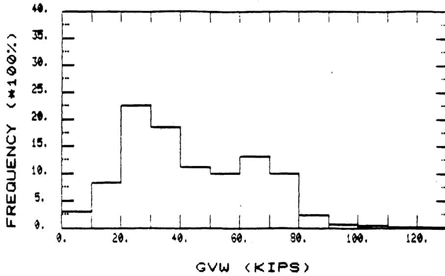
Fig. 2 GVW Distribution for Bridge 1
