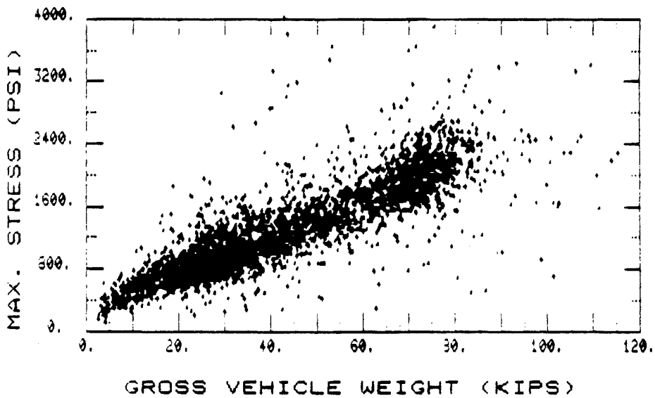
Fig. 5 Maximum Stress vs GVW - Bottom Flange - Midspan of First Interior Girder of Bridge 1
