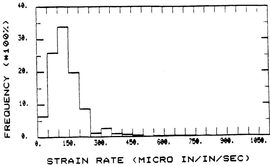
Fig. 4 Strain Rate Distribution - Bottom Flange - Midspan of Fascia Girder of Bridge 1
