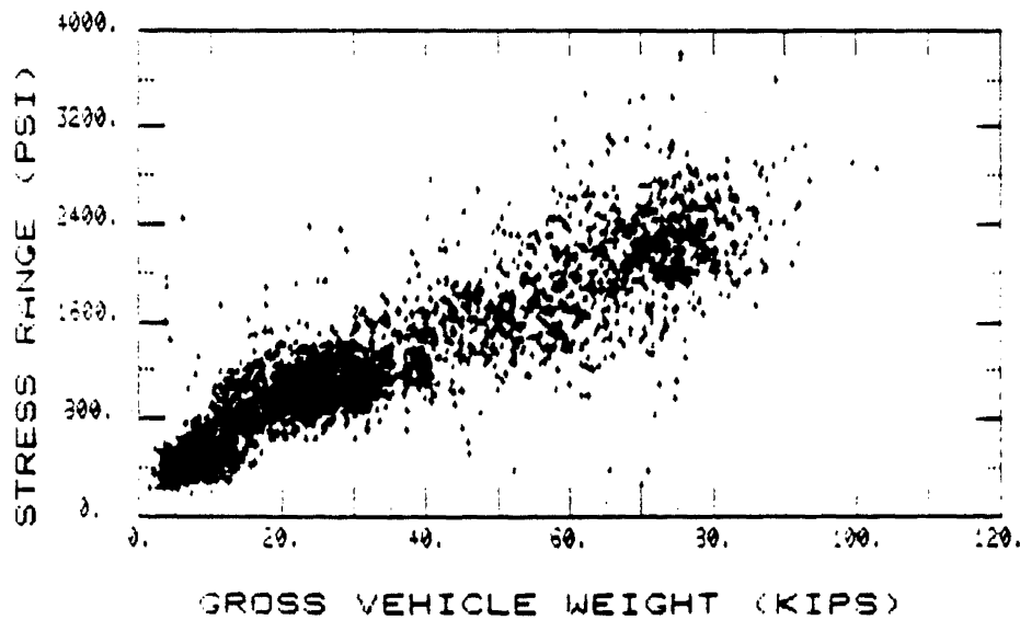
Fig. 7 Stress Range vs GWW - Bottom Flange - Midspan of First Interior Girder of Bridge 3
