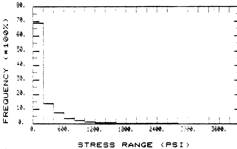
Fig. 3 Stress Range Distribution - Bottom Flange - Midspan of First Interior Girder of Bridge 1
