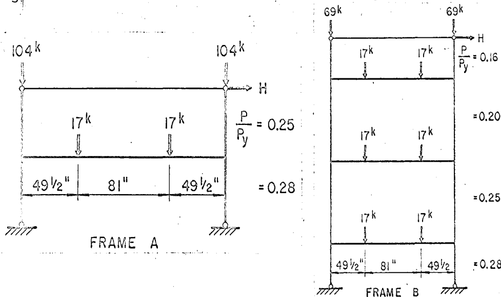
Fig. 3 Loads and Axial Load Ratios for Test Frames
