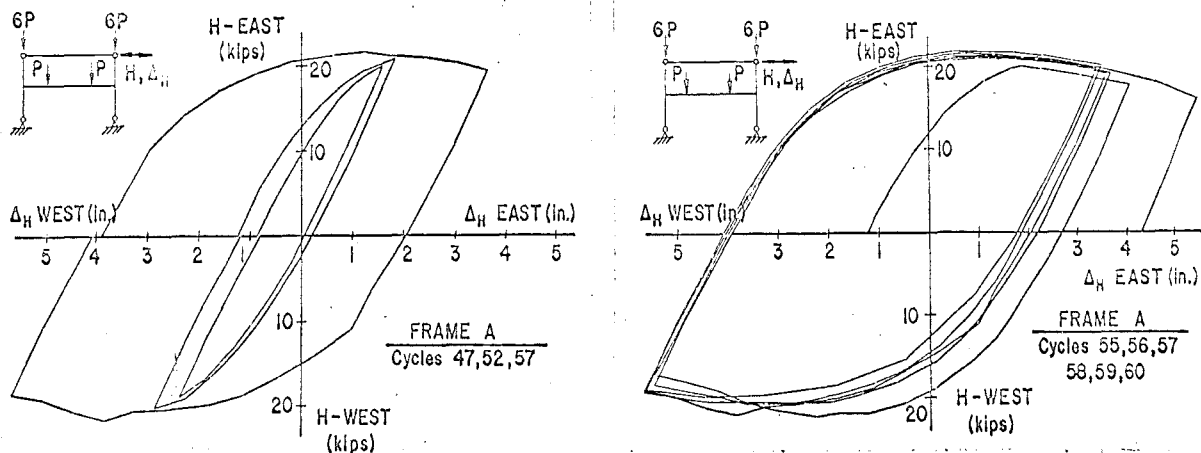
Fig. 8 Selected Load-Deflection Curves and Stability of Load-Deflection Curves for Frame A
