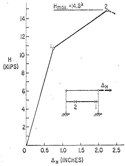
Fig. 4a Load-Deflection Curve for Frame A
