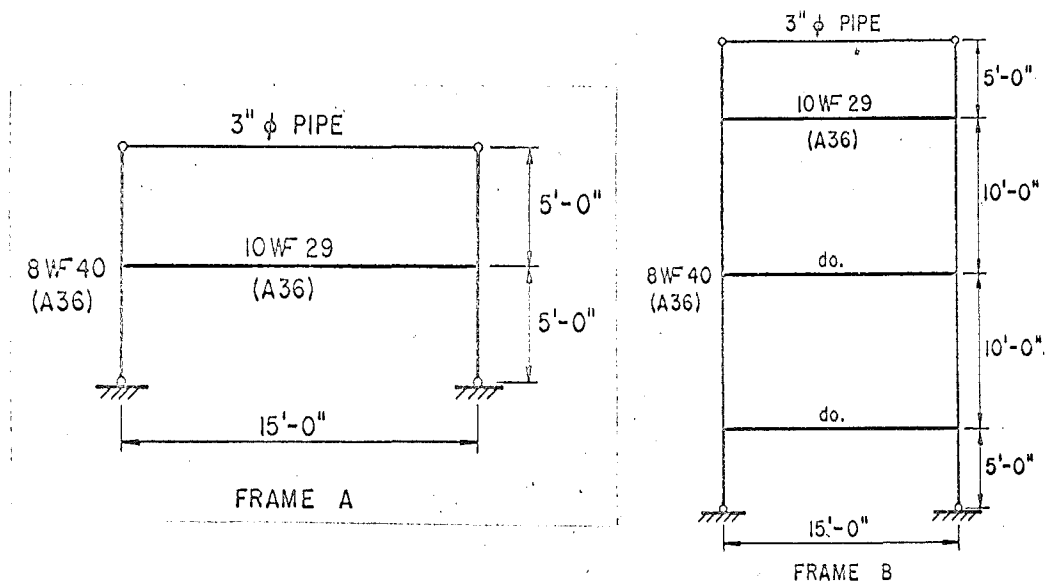
Fig. 2 Geometry and Member Sizes for Test Frames
