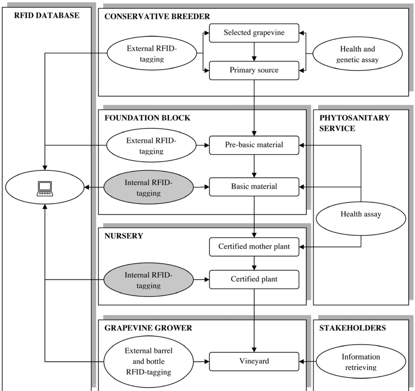
Fig. 1 - Data flow within RFID-tagged grapevine production chain.
