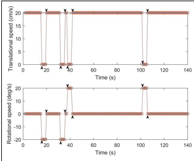
Figure 8. Offline evaluation results of the predicted actions.
