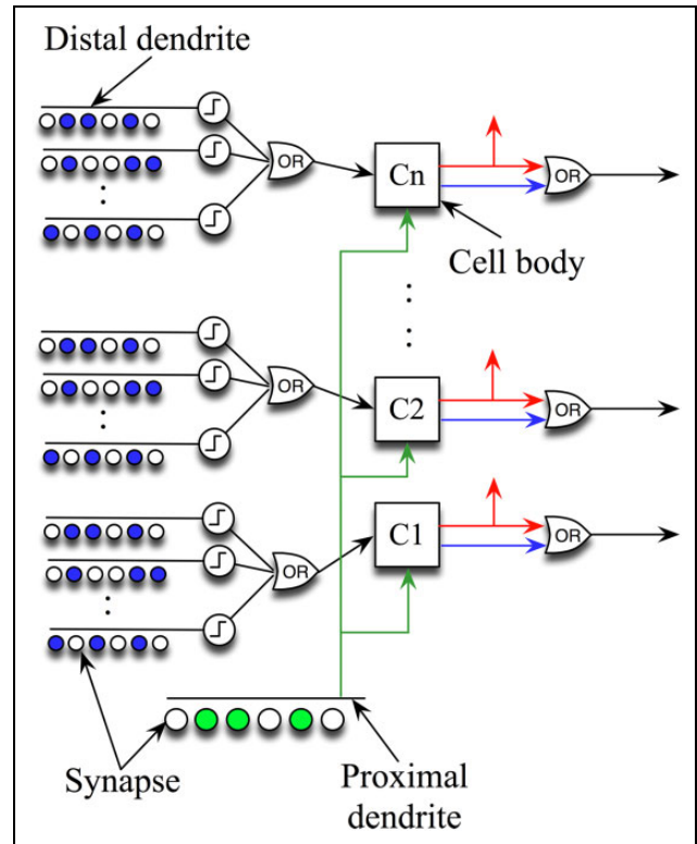
Figure 3. Components of an HTM cell. HTM: hierarchical temporal memory.
