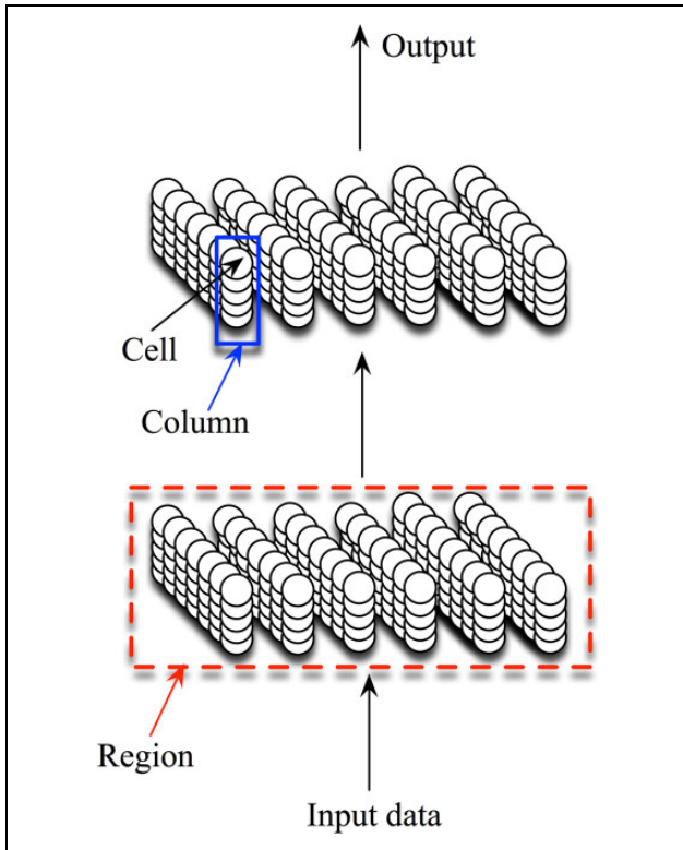
Figure 1. Structure of a typical HTM neural network. HTM: hierarchical temporal memory.
