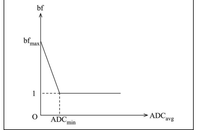
Figure 4. Function for updating the bf . bf : boost factor.
