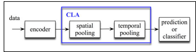
Figure 2. Workflow of an HTM application. HTM: hierarchical temporal memory.
