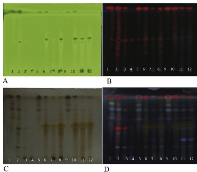
Figure 2. TLC analysis of extracts of A. altilis , A. heterophyllus and A. camansi . Silica gel F254 TLC was used as stationary phase and chloroform:methanol (9:1, v/v) as mobile phase. Detection under (A) UV 254 nm, (B) UV 365 nm, (C) heating TLC plate at 105 °C for 5 min after spraying 10% sulfuric acid and (D) observed under UV 365 nm after using spray reagent and heated. Sample: (1) hexane extract of A. heterophyllus , (2) DCM extract of A. heterophyllus , (3) methanol extract of A. heterophyllus , (4) 80% ethanol extract of A. heterophyllus , (5) hexane extract of A. altilis , (6) DCM extract of A. altilis , (7) methanol extract of A. altilis , (8) 80% ethanol extract of A. altilis , (9) hexane extract of A. camansi , (10) DCM extract of A. camansi , (11) methanol extract of A. camansi , (12) 80% ethanol extract of A. camansi .
