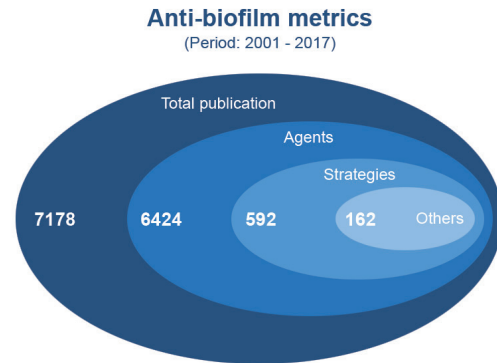
Fig. 5: publication metrics in the anti-biofilm field. The search was performed in the PubMed database ( www.pubmed.com ) on April 1st, 2018, using the keywords “anti-biofilm”, “anti-biofilm agents”, and “anti-biofilm strategies”, and only papers published in English containing these words were selected for analysis. The graphic shows the number of publications in these biofilm arenas during the period 2001-2017, which is the most representative period for publications on biofilms (Fig. 4).
