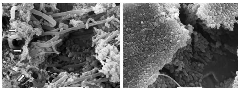
Fig. 3: polymicrobial biofilms detected on orthodontic appliances visualised by scanning electron microscopy (SEM). The SEM images reveal the presence of different microbial groups, including bacteria and fungi, and an extracellular matrix (arrows). Bars, 5 \mu m.
