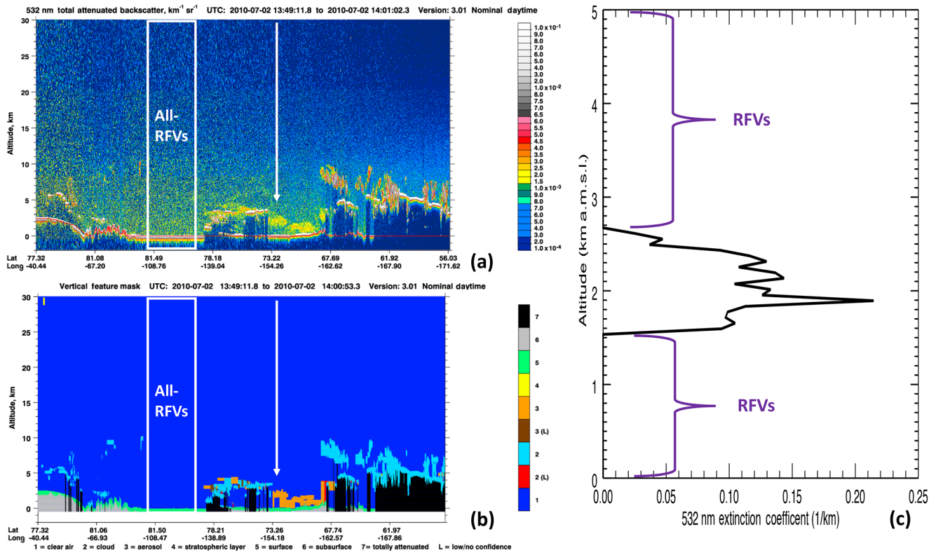
Figure 1. For data collected during the daytime on 2 July 2010 over the Arctic, browse image curtain plots of CALIPSO (a) 532 nm total attenuated backscatter ( \text{km}^{-1} \text{sr}^{-1} ) and (b) corresponding vertical feature mask (VFM). The white box represents an example segment of the granule for which range bins in the associated level 2 (L2) aerosol extinction coefficient profile are all retrieval fill values (RFVs), as the VFM classified these bins as either surface (green) or clear-air (blue) features. The white arrow indicates a column in which some aerosol has been detected (orange), and the resultant L2 aerosol extinction profile for this column is shown in (c).
