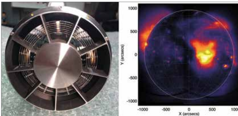
► The FOXSI X-ray mirror (left) and an X-ray image of the Sun captured by the Photon Energy Imager in soft X-rays (PhoEnIX), one of FOXSI-3's new cameras (right).
