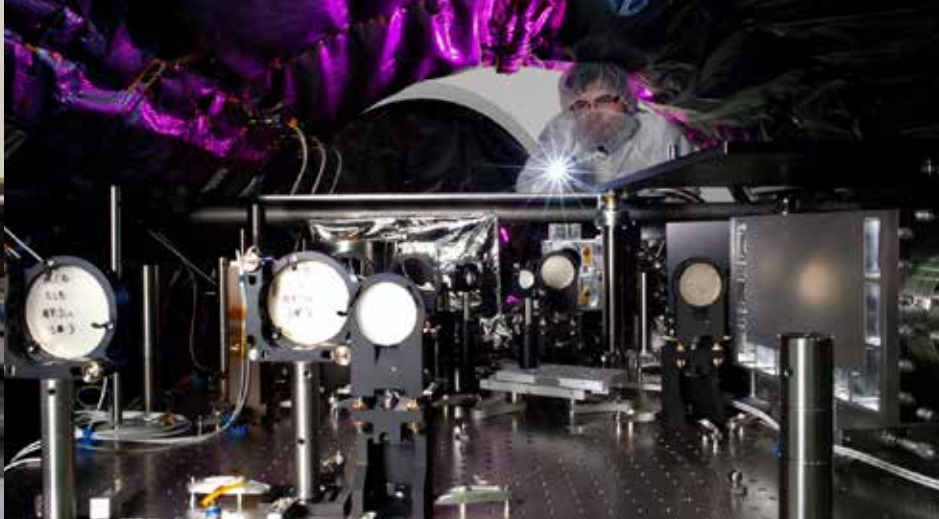
▶ Left: The Decadal Survey Testbed inside the vacuum chamber at the High Contrast Testbed Facility at the NASA Jet Propulsion Laboratory (JPL). Right: Manager of the testbed facility, Dr. Camilo Mejia Prada, looks into the vacuum chamber to view an ongoing coronagraph experiment.
