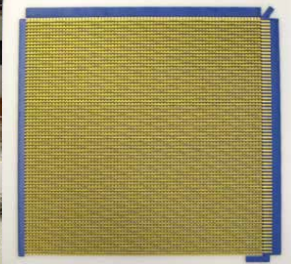
▶ Team members inspecting a 20 cm atomic layer deposited microchannel plate (left). Cross strip imaging readout anode (right).
