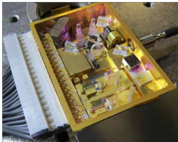
► Final product of the Phase 1 master oscillator package.
