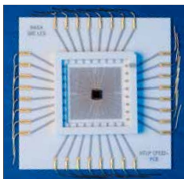
► Packaging technology able to survive the 465°C, 92-atmosphere, caustic environment of the Venus surface is enabling new planetary exploration.
