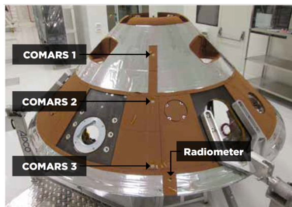
Figure 1. Location of COMARS sensors [1]
