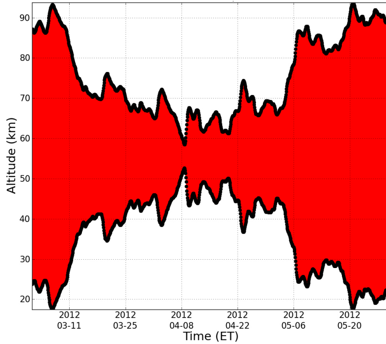
Figure S2. Orbital periapsis and apoapsis during GRAIL's PM. Altitudes are relative to the lunar mean radius of 1737.4 km (26) as measured by the Lunar Orbiter Laser Altimeter (47).
