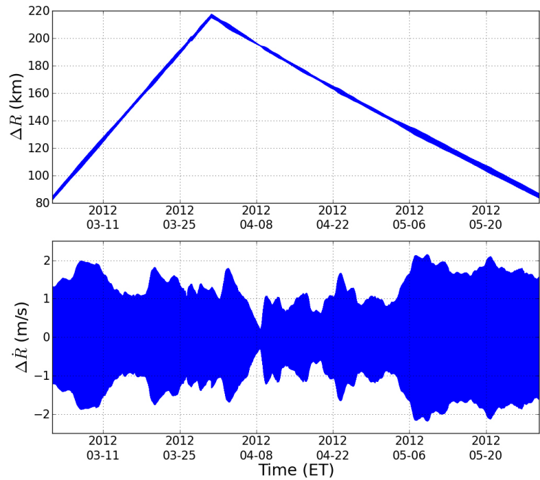
Figure S3. Spacecraft separation distance ( \Delta R ; top) and drift rate ( \Delta \dot{R} ; bottom) of the GRAIL spacecraft during the PM.
