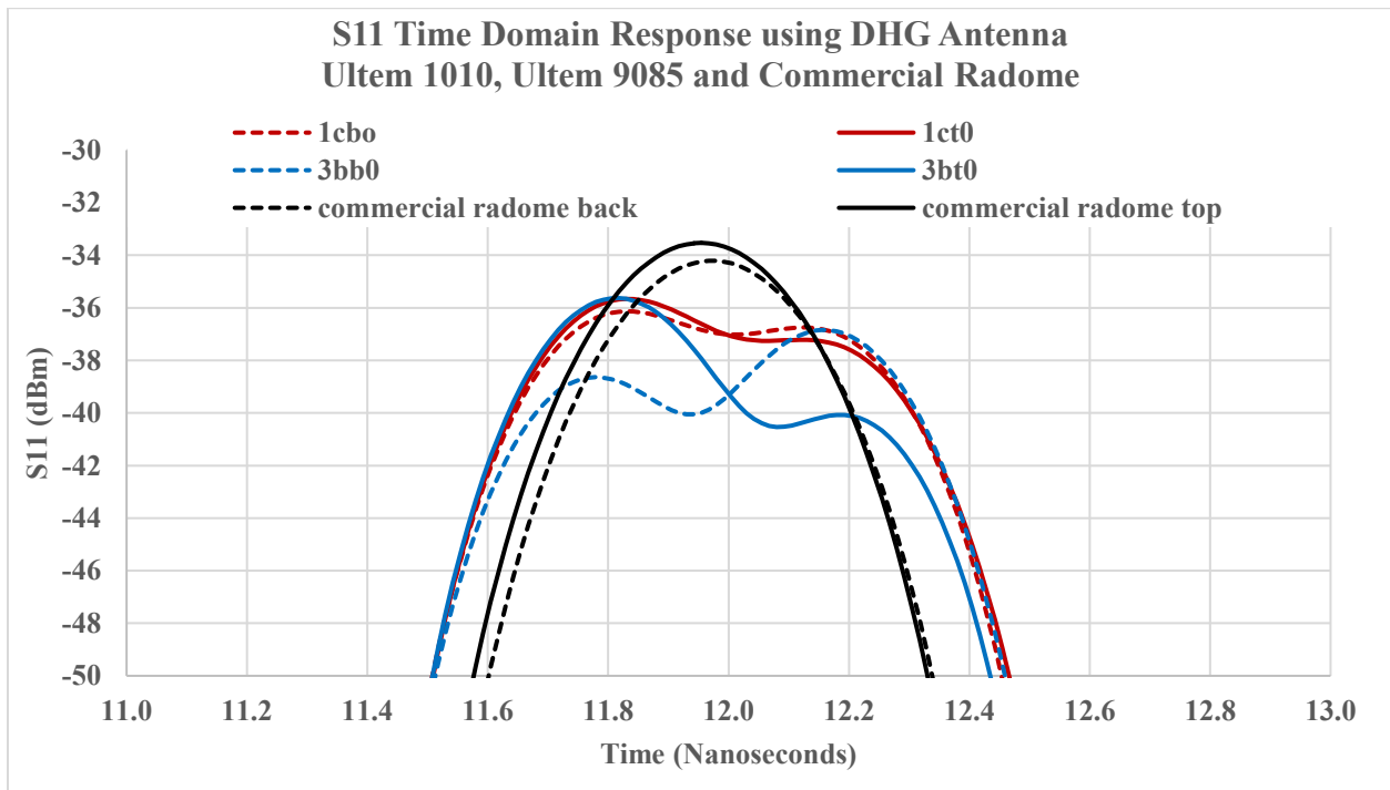
Figure 12. S11 Time Domain Response of Ultem 1010, 9085 & Commercial Radome using DHG Antenna.
