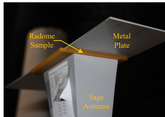
Figure 1. Ultem 1010 and metal plate covering Sage antenna aperture for transmission measurement.
