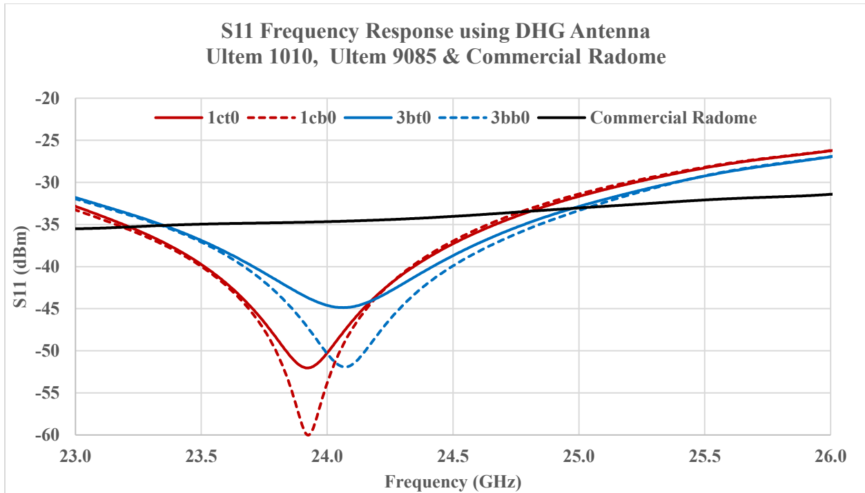
Figure 11. S11 Frequency Response of Ultem 1010, 9085 & Commercial Radome using DHG Antenna.
