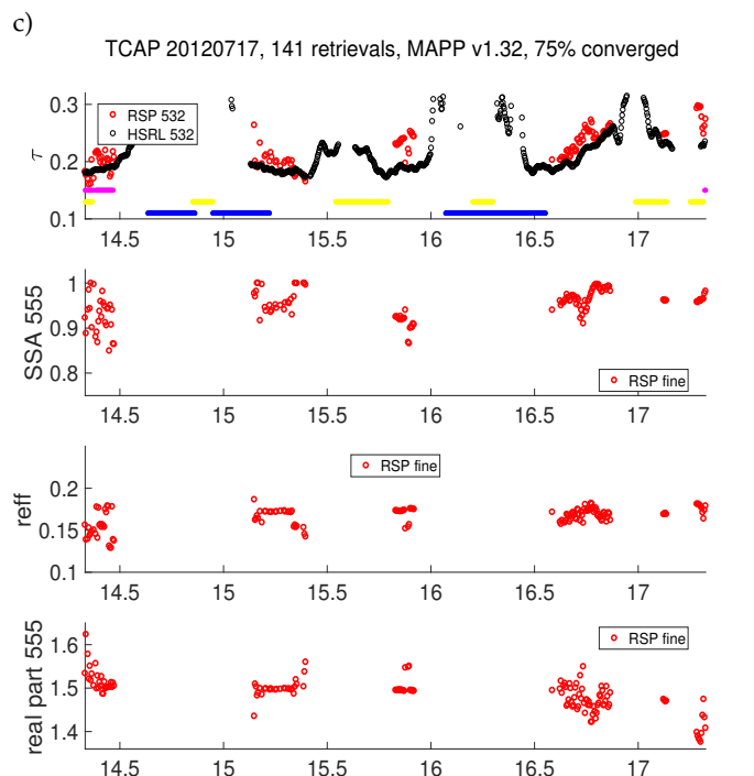
Fig. 7. TCAP 07/17/2012. a) HSRL direct measurement of extinction \text{km}^{-1} at 532 nm. b) HSRL-1 aerosol typing product. c) Atmosphere retrieval results from the RSP instrument for this entire day. RSP MAPP 532 nm aerosol optical depth and aerosol microphysics retrievals vs HSRL-2 532 nm aerosol optical depth (direct measurement) and HSRL-2 aerosol microphysics products for a time-series of retrievals between 14.5 UTC and 17.5 UTC on 7/17/2012. Aerosol products: (i) optical depth, (ii) single-scattering albedo, (iii) effective radius, (iv) real part of the refractive index. The following masks are also displayed, where the color indicates the presence of: clouds-above-aircraft (cyan), aircraft not at cruising altitude (magenta), aircraft turns/course corrections (yellow), and clouds below the aircraft (blue).
