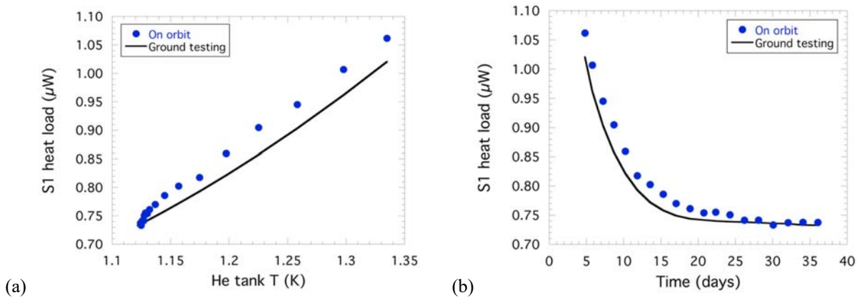
Figure 7. Heat load on stage 1 for each ADR cycle on orbit as a function of (a) helium tank temperature and of (b) time on orbit. The solid lines indicate the expected heat loads at the indicated tank temperature or time based on ground testing.
