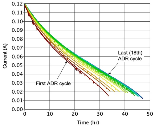
Figure 5. Demagnetization curves for stage 1 for the 18 cycles completed on orbit. Time is from the first crossing of 50 mK after recycling. The exponential approach of the helium tank to its steady-state temperature gave rise to a gradual increase in hold time with each cycle.
