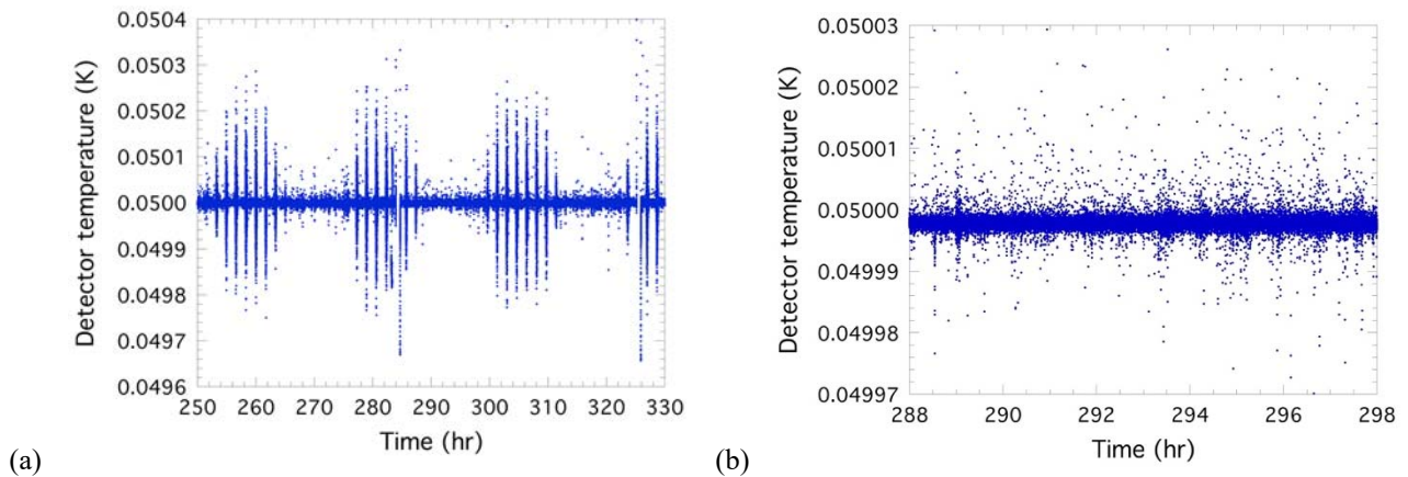
Figure 6a. Detector array temperature (a) showing the effect of high-energy particles during passes through the South Atlantic Anomaly, and (b) when Hitomi was outside the region of the SAA.
