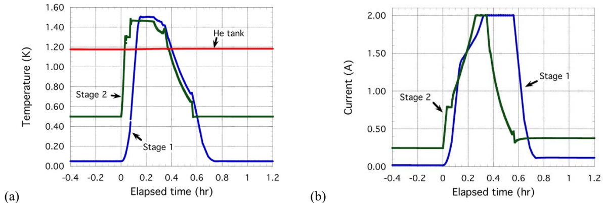
Figure 3. Temperatures (a) and magnet currents (b) during an ADR recycle (ground test data).
