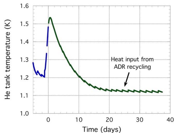
Figure 8. Helium tank temperature from shortly before launch through to the end of operations on day 38. The increase leading up to launch was due to closure of the vent valve and periodically turning off the cryocoolers.
