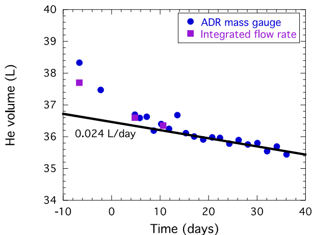
Figure 9. Helium volume as determined from ADR recycles, compared to a direct measurement after the final top-off that was then integrated to reflect boiloff loss as the helium cooled. The solid line represents a loss rate of 0.024 L/day.
