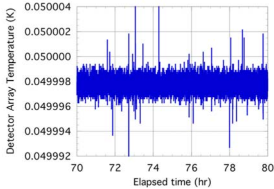
Figure 4. Typical detector array temperature during ground testing at 50 mK.
