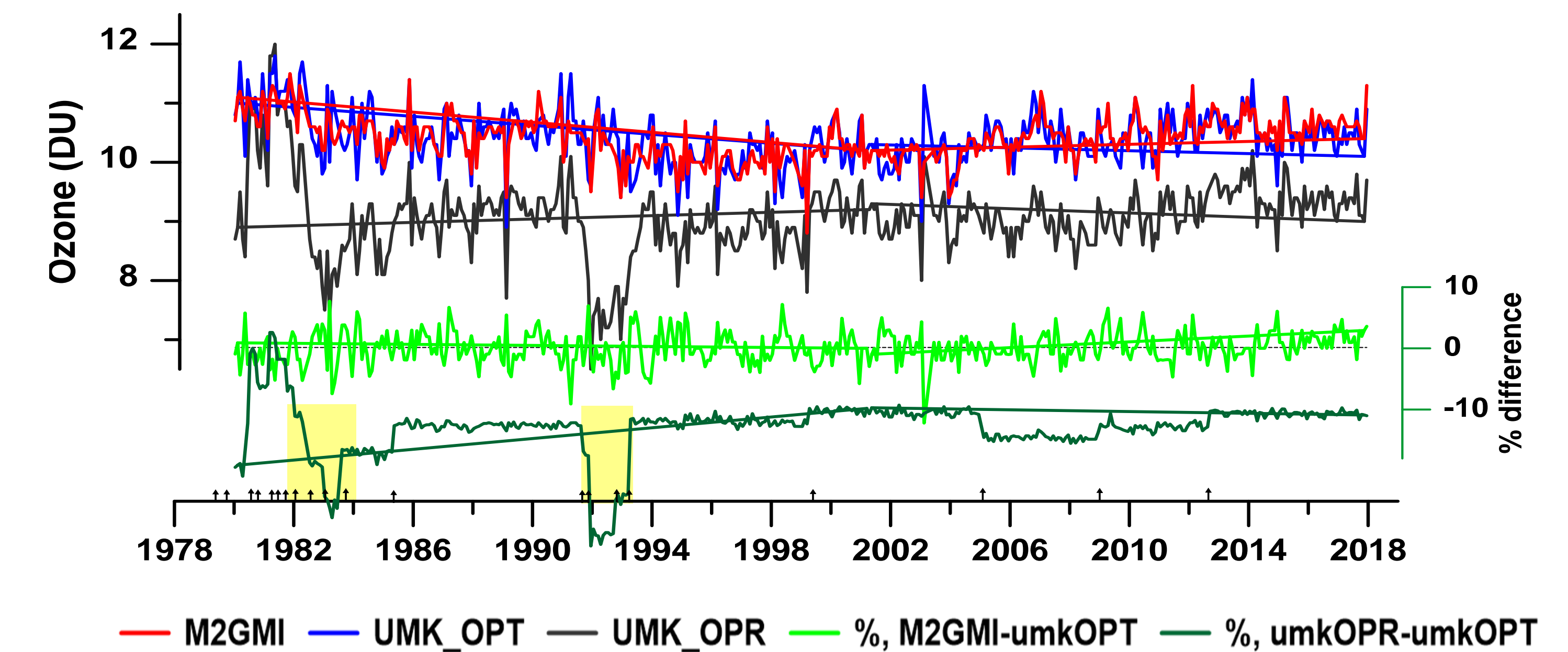
Figure 4. The time series of ozone at Boulder in Umkehr layer 8 (2-4 hPa). Operational Umkehr (black), Optimized Umkehr (blue) and M2GMI (red) data are shown as monthly averages. Difference between Optimized and Operational Umkehr data is shown as a dark green line. The percent difference between optimized Umkehr and M2GMI model is shown as a light green line. The arrows at the bottom indicate dates of Dobson calibrations and instrument replacements.
