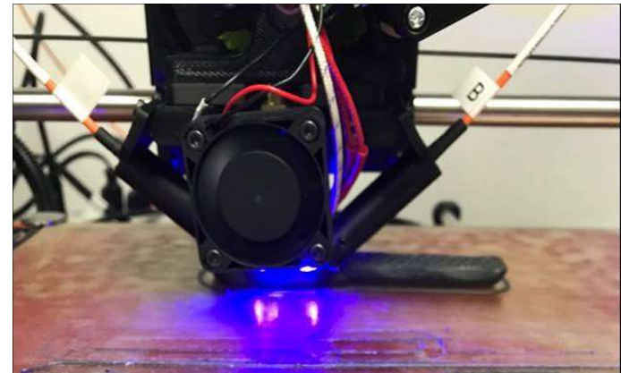
Retrofitted FFF head with laser printing a PEEK wrench. Image credit: Actuated Medical, Inc.
