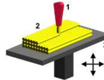
Illustration of the FFF process
