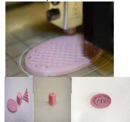
FFF prints using reclaimed anti-static bagging film with reversible cross-linking additive (image from Cornerstone Research Group)
