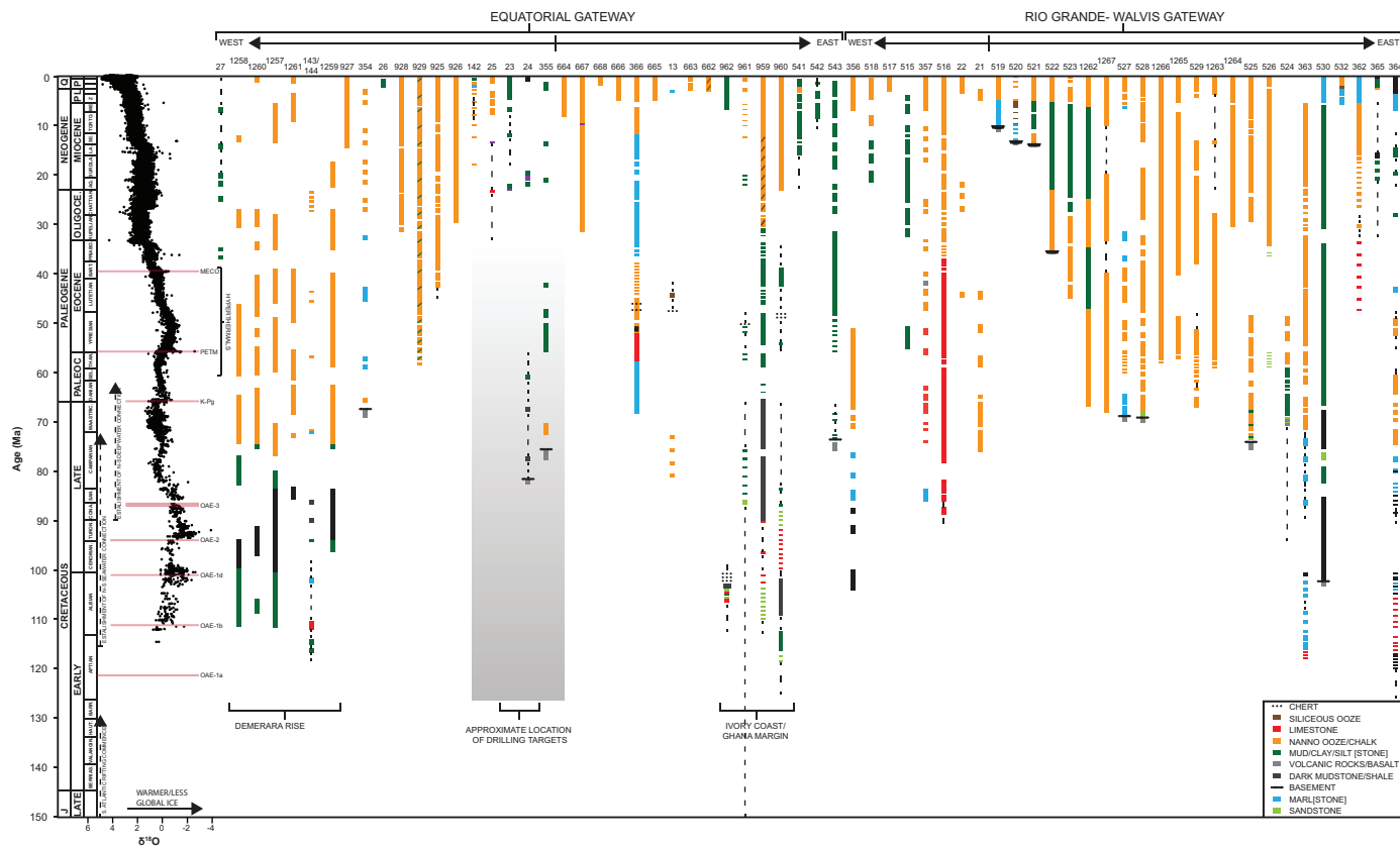
Figure F4. Existing DSDP/ODP/IODP drilling in the equatorial and South Atlantic; note very limited sampling of the Late Cretaceous (compiled by Alex Dickson; benthic \delta^{18}O record is from Zachos et al. [2001] and Friedrich et al. [2012]).
