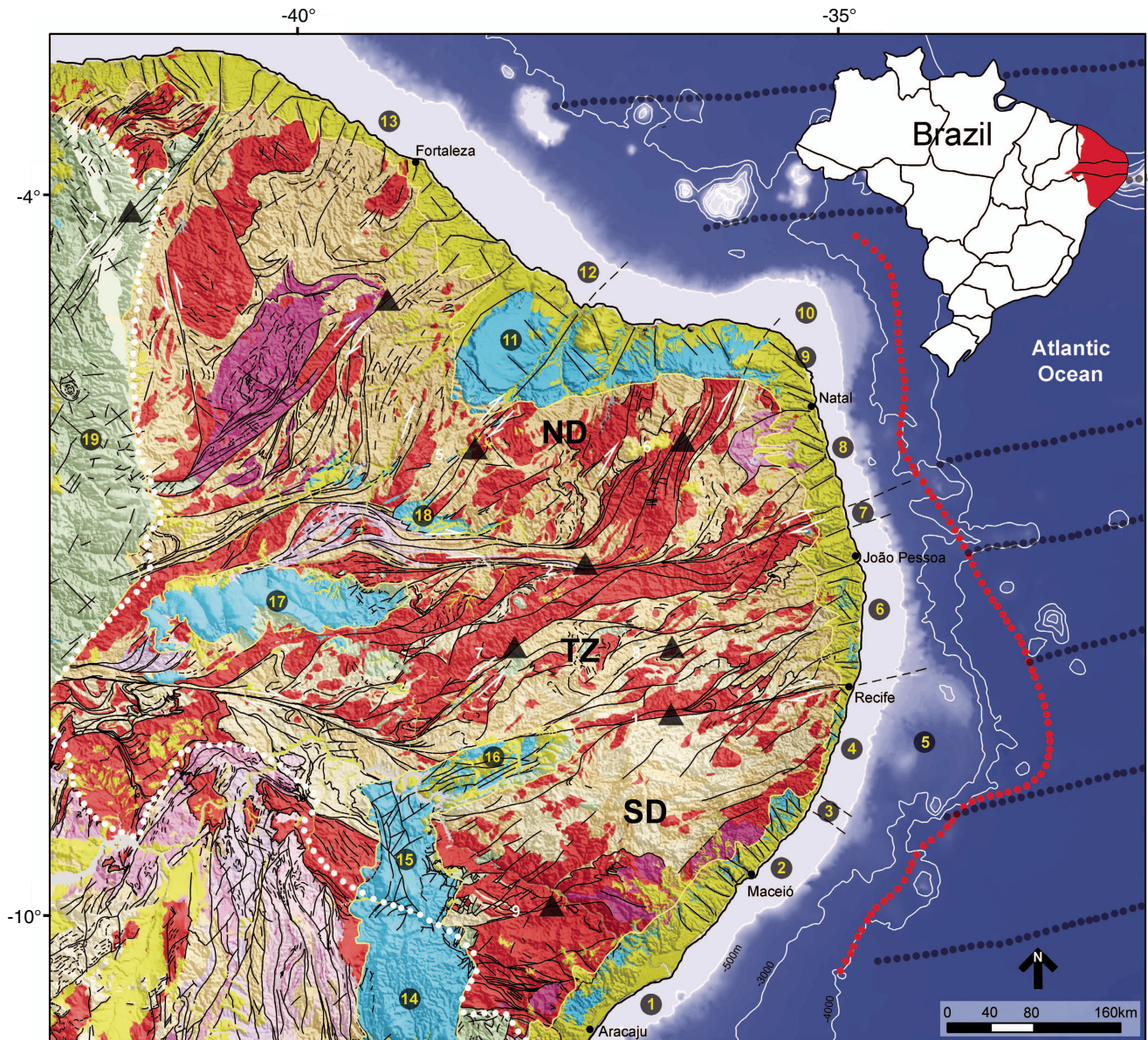
Figure F2. Borborema Province, northeast Brazil. Geological map over a digital elevation model, including sedimentary basins, basement rock ages, and the main shear zones and lineaments (Brazilian Geological Survey databank). Red dotted line = estimated position of continent–ocean boundary (COB) (after Blaich et al., 2008; Magalhães et al., 2014). S.Z. = sheer zone, Plataf. = platform, ND = north domain, TZ = Transversal Zone, SD = south domain.
