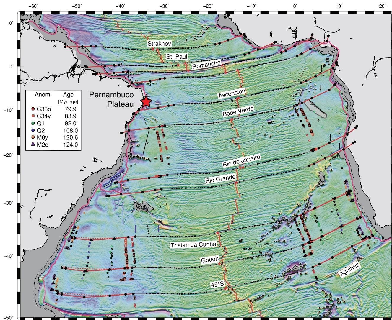
Figure F1. South and equatorial Atlantic tectonic structure superimposed on satellite-derived free-air gravity field with magnetic picks (Granot and Dymant, 2015). Red lines are flowlines calculated on the basis of the new Granot and Dymant (2015) stage rotations. The red star indicates the location of the Pernambuco Plateau.
