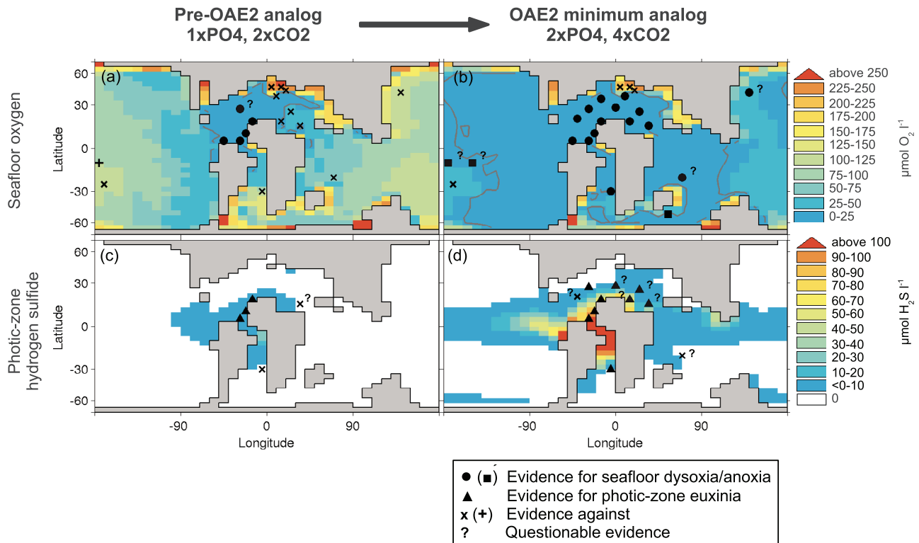
Figure F9. Model-data reconstruction of marine biogeochemistry before and during OAE2. (A, B) Seafloor oxygen condition showing modeled oxygen concentration in color. Gray contour = modeled oxygen concentration of 10 mmol O 2 l -1 , delimiting the region of seafloor dysoxia/anoxia. (C, D) Photic zone free hydrogen sulfide (H 2 S) condition showing modeled H 2 S concentration in color for 80–200 m depth. Euxinia is defined by the occurrence of free hydrogen sulfide (H 2 S > 0, in white). Note focus of euxinia in the equatorial and South Atlantic (Monteiro et al., 2012).
