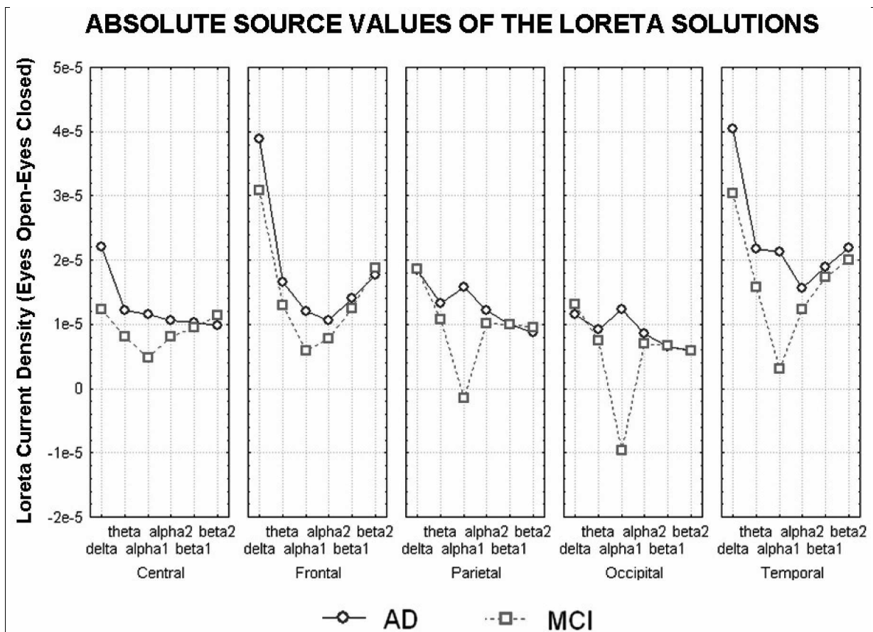
Fig. 2. Absolute source values of the LORETA solutions (eyes-open minus eyes-closed) in MCI and AD subjects for the delta, theta, alpha 1, alpha 2, beta 1, and beta 2 bands. (Colors are visible in the electronic version of this article at http://dx.doi.org/10.3233/JAD-2010-100798 )
