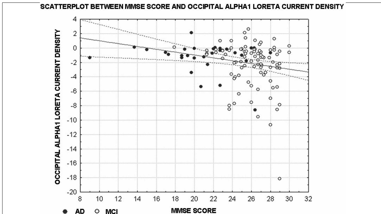
Fig. 4. Scatter plots relative to the results of a correlation analysis between MMSE and occipital alpha 1 sources of EEG rhythms (eyes-open minus eyes-closed) in the MCI and AD subjects as a whole group. (Colors are visible in the electronic version of this article at http://dx.doi.org/10.3233/JAD-2010-100798 )
