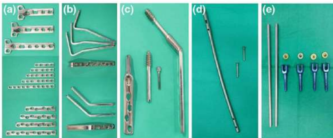
Fig. 5 Various types of implants used for traumatic purposes: a plates in various types and sizes; b angled-blade plate, commonly used for proximal or distal femoral fractures; c dynamic hip screw, widely used for cases in proximal femoral fracture; d interlocking nail, suitable for long bone fracture of lower extremity; and e pedicle screw and rod, used for posterior spine stabilization (Courtesy of Dr. Soetomo General Hospital, Surabaya)
