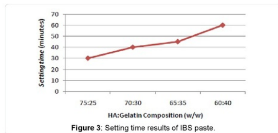
Figure 3: Setting time results of IBS paste.
