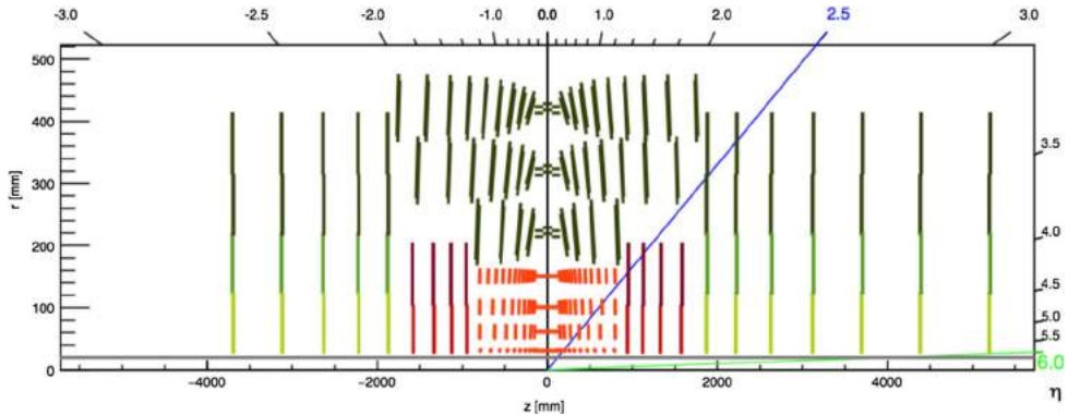
Fig. 7.29. r – z view of the all-silicon FCC-eh tracking detector; left: direction of the electron beam (backward), right: direction of the hadron beam (forward). The radius extension is 0.5 m to facilitate a dipole radius that is not too large and to limit the area of silicon required.
