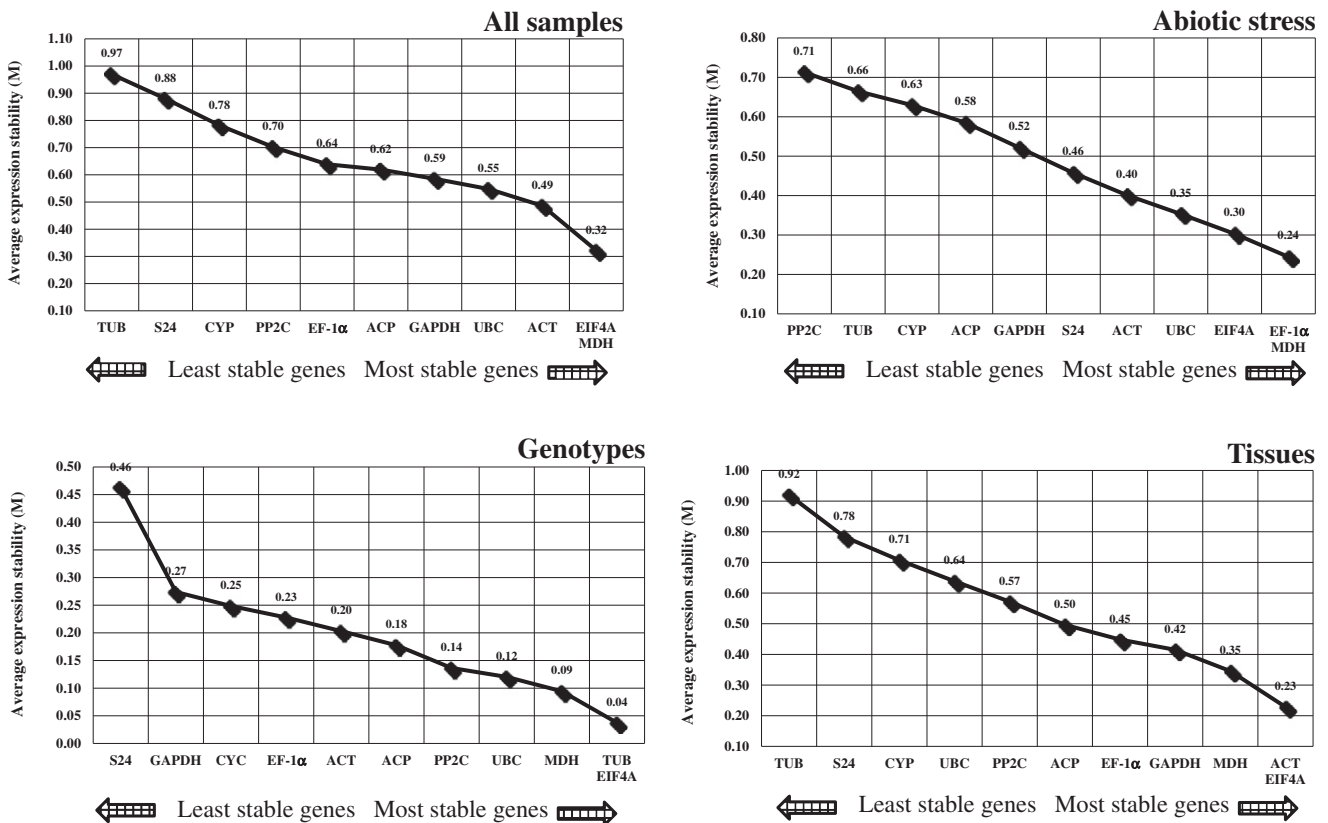
Fig. 3. Gene expression stability and rankings of eleven candidate reference genes using geNorm software. The average expression stability (M) was calculated following stepwise exclusion of the least stable gene across all the samples within an experimental set, the lowest M value indicates the most stable gene, while the highest value represents the most variable gene.
