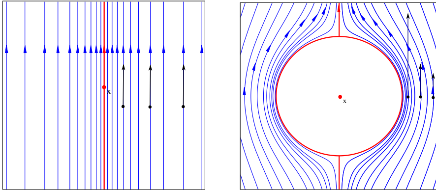
FIGURE 5. Lift of orbits of a vector field on \mathbb{R}^2 (left) to \text{Bl}(\mathbb{R}^2, \{x\}) \cong S^1 \times [1, +\infty) (right).
