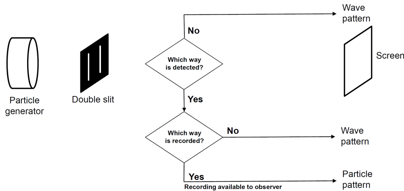
Figure 5: Detecting but not recording “which-way”
