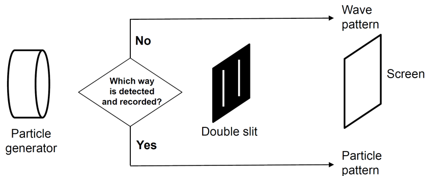
Figure 1: The classical double slit experiment [17, 2] with which-way detected before or at the slits. We write “wave pattern” for interference pattern, and “particle pattern” for non-interference pattern.
