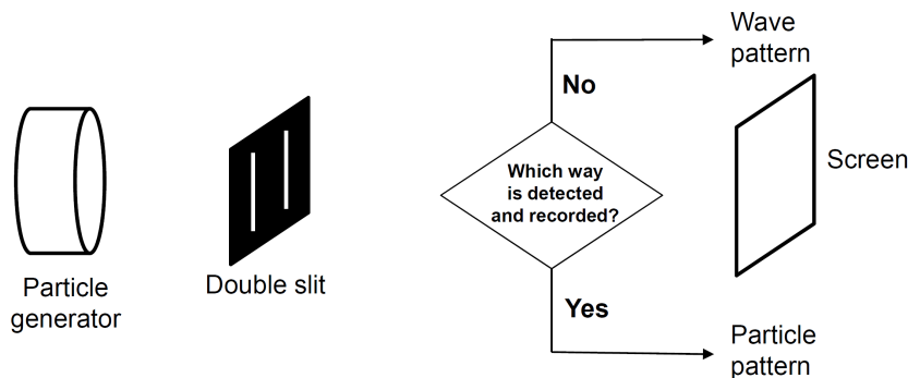
Figure 2: The delayed choice experiment [50, 23]. The choice of whether or not to detect and record which-way data is delayed until after each particle has passed through a slit but before it reaches the screen.
