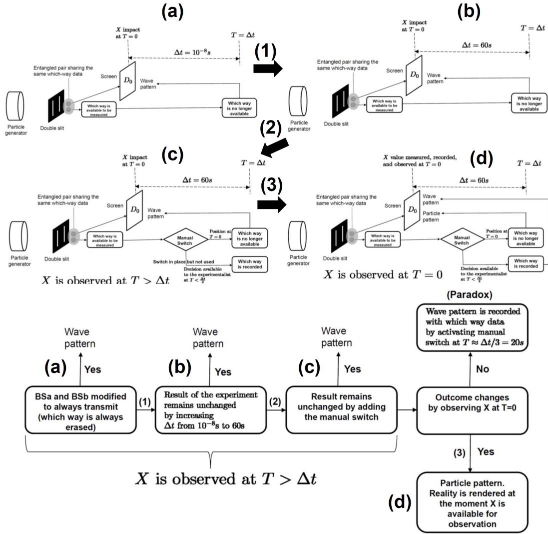
Figure 8: Testing the role of the observer
