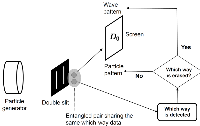
Figure 3: The delayed choice quantum eraser experiment [40, 25]. Which-way data is collected before, at, or after each particle has passed through a slit, however, this which-way data may be erased before the particle hits the screen. This experiment is sometimes called a delayed erasure experiment since the decision to erase is made after the particle has passed through a slit (chosen one path or the other).
