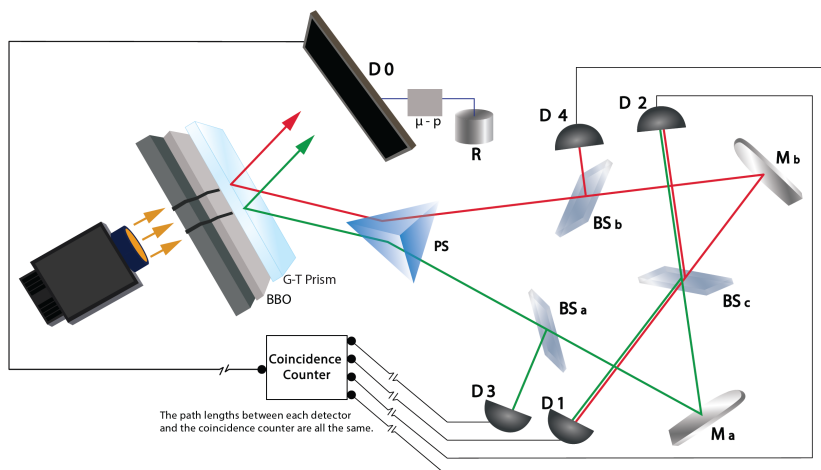
Figure 4: The delayed choice quantum eraser experiment set up as described in [25]. The microprocessor ( \mu -p) represents an addition to the original experiment and will be discussed in subsections 4.4 and 4.5.
