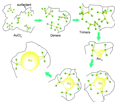
Figure 13. Formation of gold nanoparticles through \text{Au}_2\text{Cl}_6 . Reprinted with permission from ref 58. Copyright 2010 American Chemical Society.
