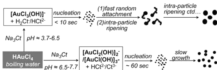
Figure 8. Schematic illustration of two reaction pathways for the formation of gold nanoparticles by citrate reduction. Reprinted with permission from ref 56. Copyright 2007 American Chemical Society.
