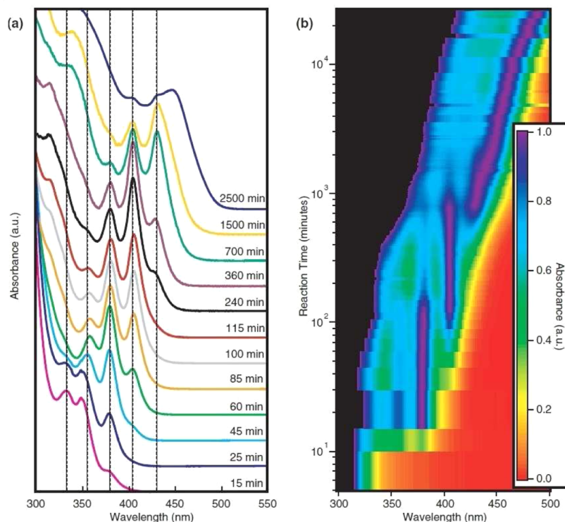
Figure 32. UV-vis absorption spectra of CdSe with time. Reprinted with permission from ref 102. Copyright 2007 WILEY-VCH Verlag GmbH & Co. KGaA, Weinheim.
