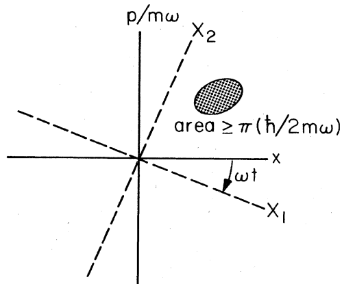
FIG. 1. "Error box" in the phase plane for a quantum-mechanical oscillator. This error box is an ellipse, with centroid at the expectation value \langle \hat{x} \rangle, \langle \hat{p}/m\omega \rangle of the position and momentum. The principal axes of the error ellipse are the eigendirections of the variance matrix
