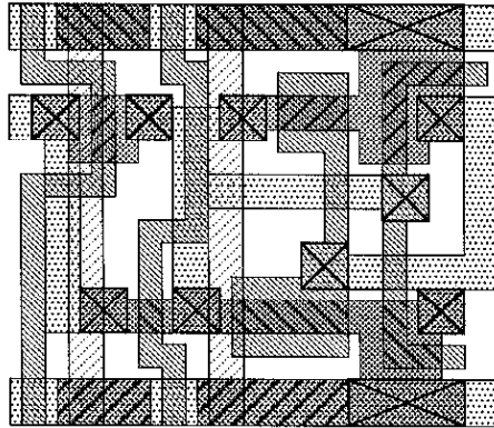
Figure 21: FIFO storage register
