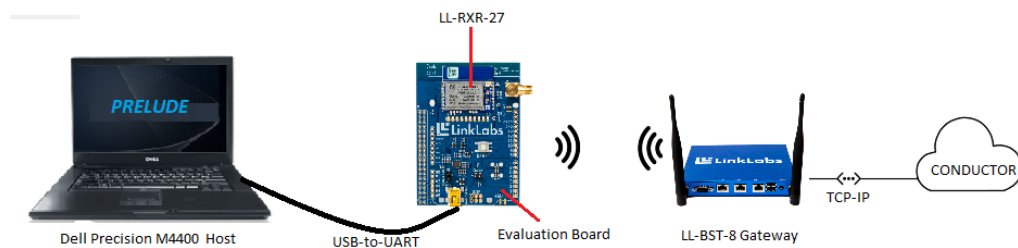
Figure 16: System architecture.
