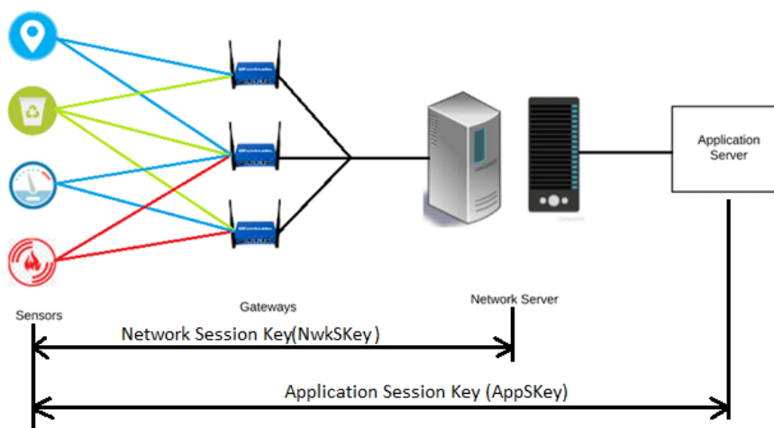
Figure 14: LoRaWAN security.
