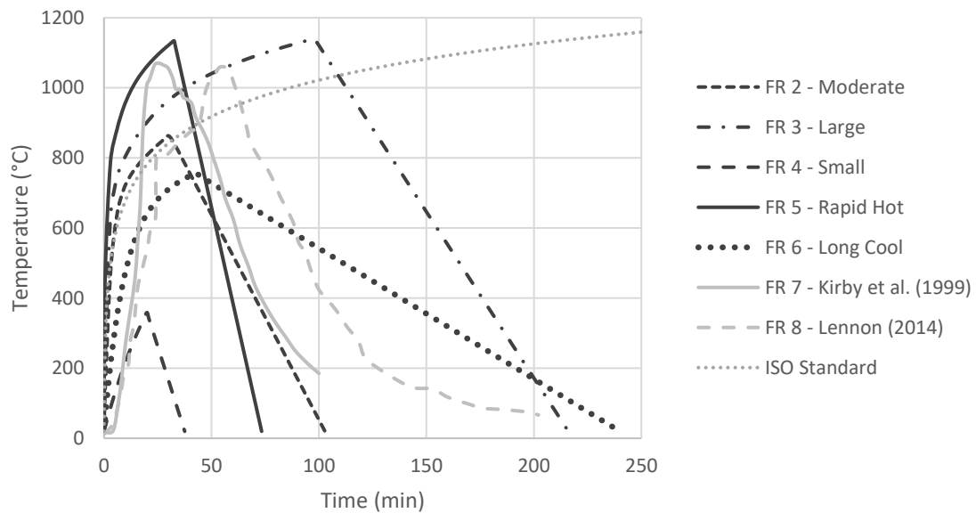
Fig. 4.2 Representative Design Fire Profiles
