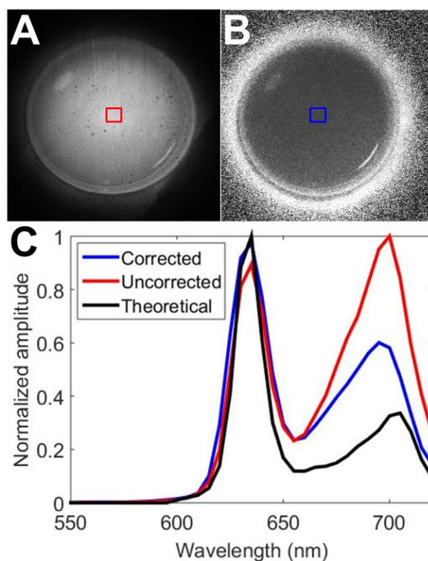
Figure 5-6: (A) Uncorrected image of PpIX in petri dish. (B) Corrected image of PpIX. (C) A theoretical spectrum of PpIX emission together with calibrated and uncalibrated spectra retrieved from regions of 20 x 20 pixels in images of a PpIX sample.
