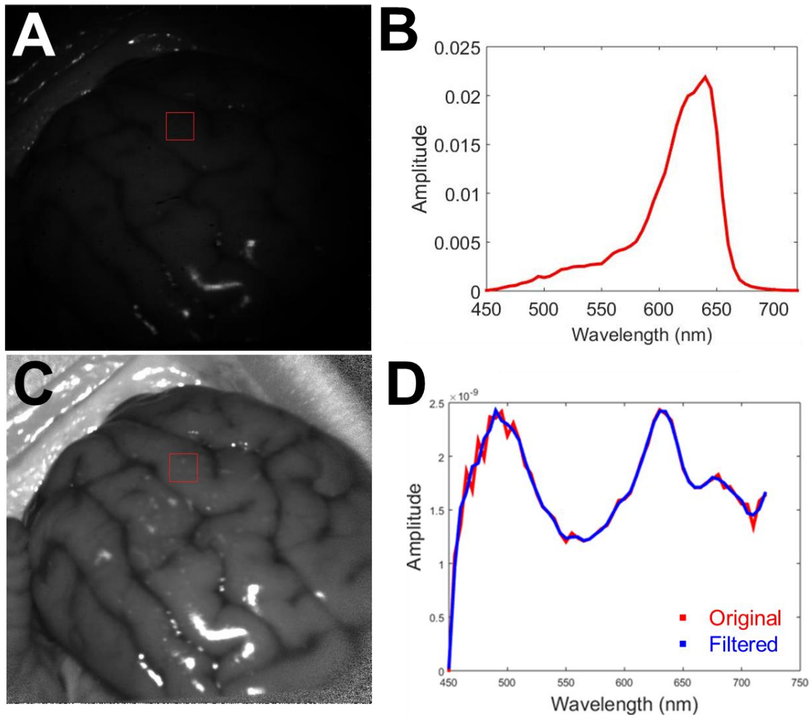
Figure 5-7: (A) Uncalibrated reflectance image of a calf brain. (B) White light reflectance spectrum obtained from the square region in (A). (C) Calibrated image of a calf brain in white light reflectance mode. (D) Filtered reflectance spectrum recovered from the red square in (C).
