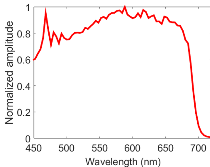
Figure 5-1: Spectrum of the microscope white lamp ( I_o ) measured with a spectrometer.
