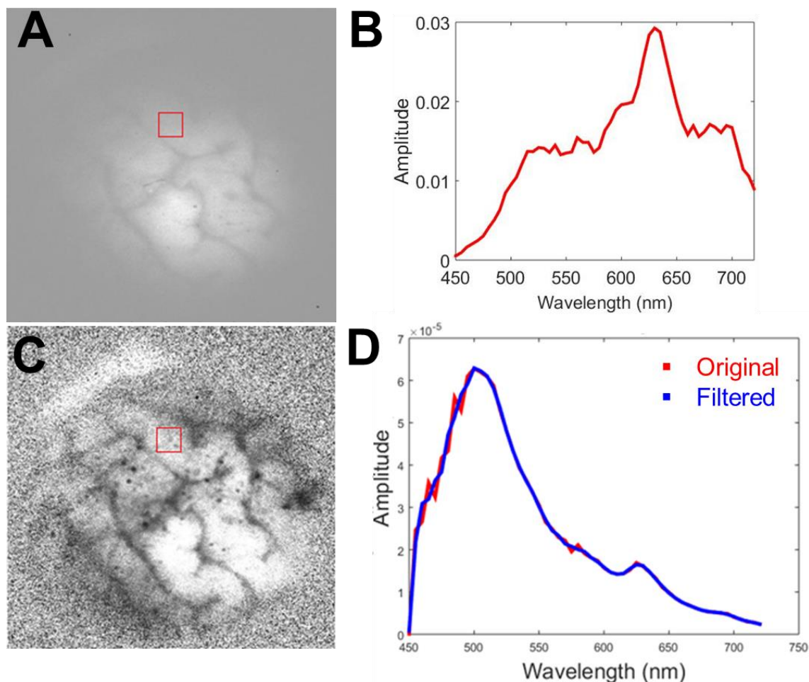
Figure 5-8: (A) Uncalibrated fluorescence image of a calf brain. (B) The average spectrum (20 x 20 pixels) of the red square region in (A). (C) Calibrated fluorescence image of a calf brain. (D) The corresponding spectrum of the square region in (C).
