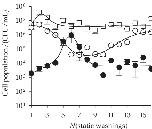
Fig. 3. Changes in the microflora during subsequent static washings prior to brining of Kalamata olives
