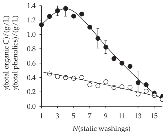
Fig. 2. Changes in the total phenolics and total organic carbon of the washwater during subsequent static washings prior to brining of Kalamata olives
