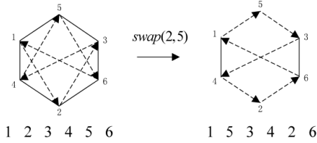
Figure 3: Illustration of swap transformation for TSP
