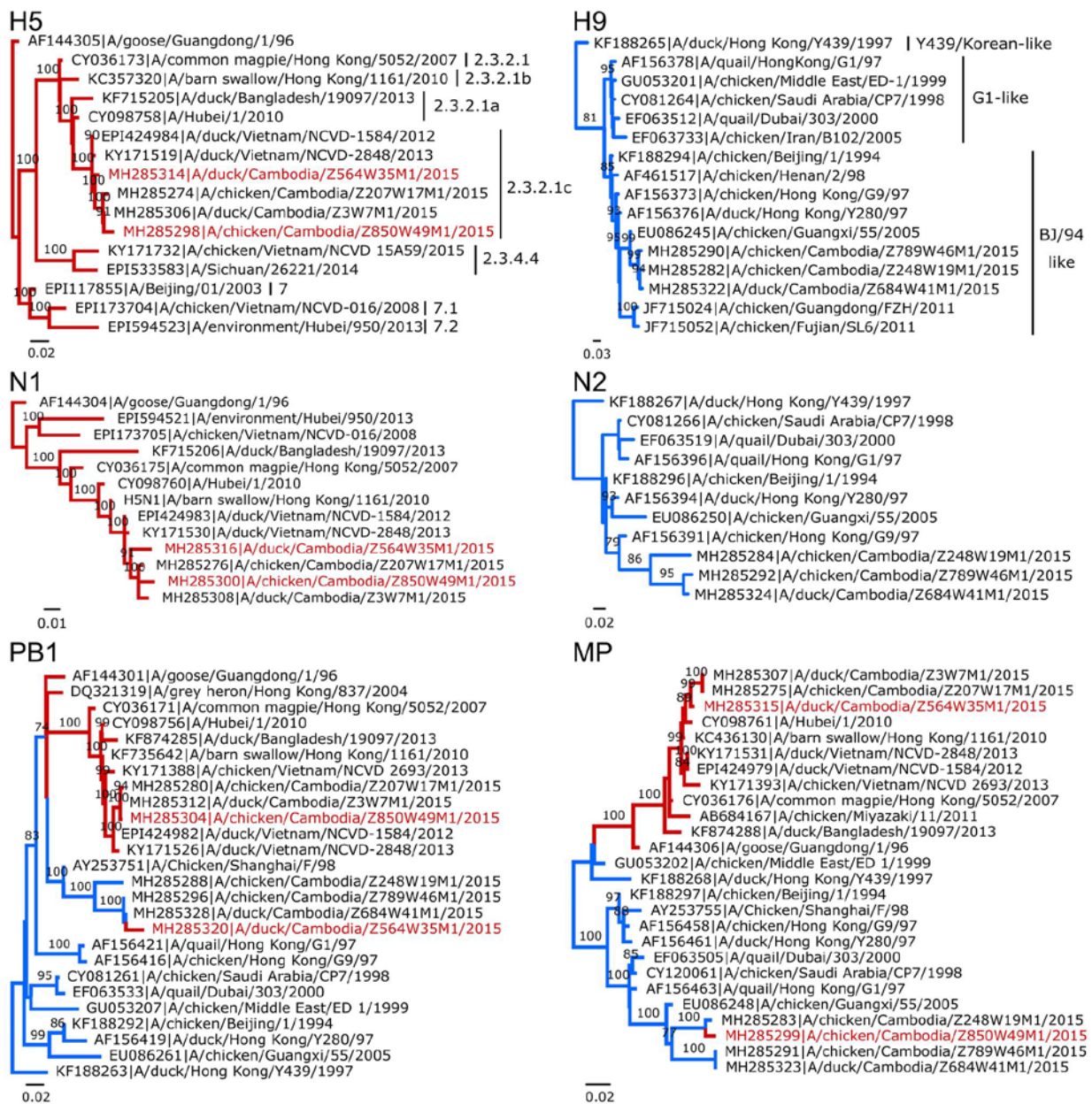
Fig. 1. Phylogenetic analysis of HA, NA, PB1 and MP genomic segments of the Cambodian A(H5N1) reassortant viruses. Trees were constructed using the maximum likelihood method based on the general time-reversible model with gamma distribution. Branches of H5 and N1 genes trees are presented in red. Branches of H9 and N2 genes trees are presented in blue. Branches of PB1 and MP genes are colour coded based on the subtype of HA genes, A(H5) viruses are red and A(H9) viruses are blue. The taxa of both Cambodian A(H5N1) reassortant strains (A/duck/Cambodia/Z564W35M1/2015 and A/chicken/Cambodia/Z850W49M1/2015) have been highlighted in red. Scale bars indicate the number of substitutions per site and bootstrap values (n = 1000) of 70 or greater are shown.
