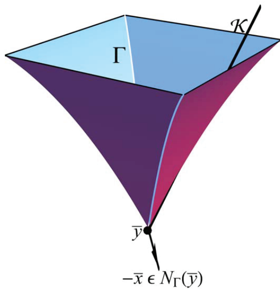
Fig. 1 Illustration of the feasible set \Gamma defined by (27) and of the critical cone \mathcal{K} .
