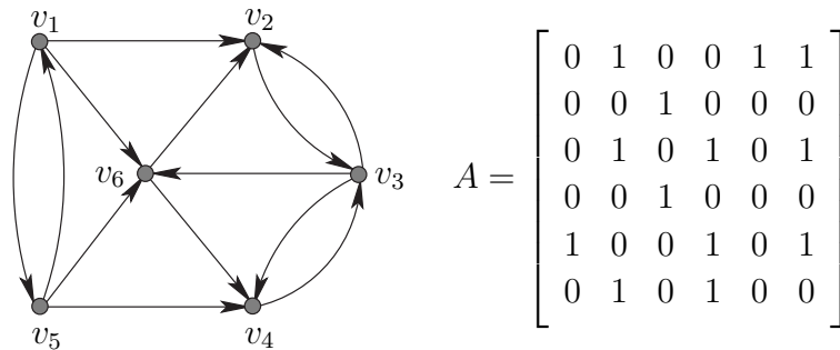
Figure 1.8: Digraph and its adjacency matrix.
