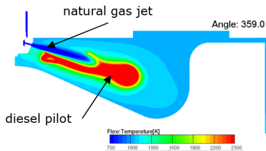
Figure 9: HPDI principle – hot gas from diesel pilot injection at the nozzle bottom ignites the methane gas jet above – as illustrated with temperature distribution calculated by CFD.
