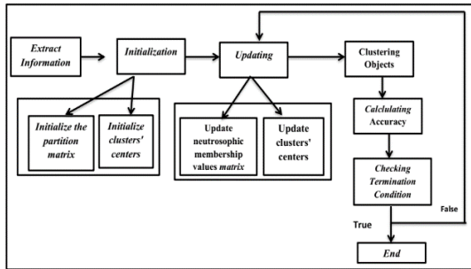
Figure 1. New Neutrosophic C-Means Clustering System
