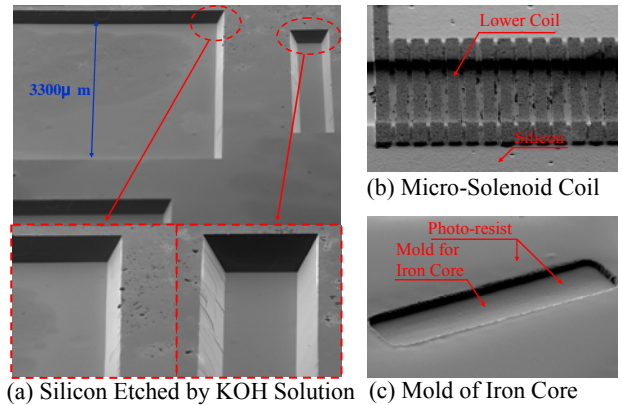
Fig. 11 A Few SEM of Fabricated Tri-axis Micro-power Receiver
