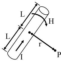
Fig. 1 Magnetic Flux Induced by A Straight Wire
