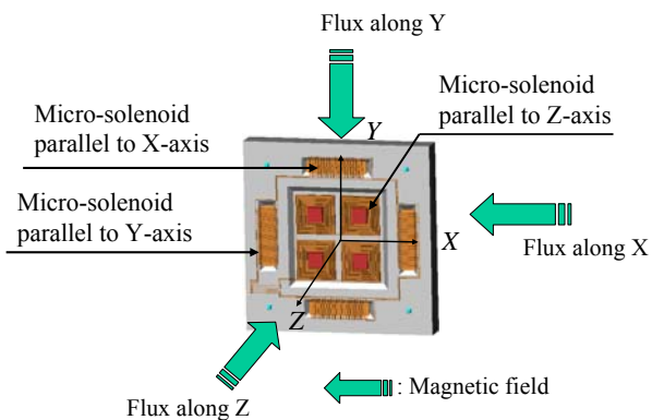
Fig. 4 Magnetic Energy and the Micro-power Receiver
