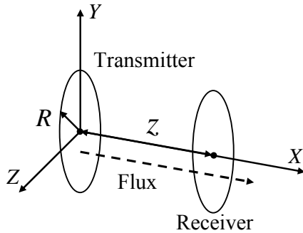
Fig. 2 Transmitter and Receiver for Wireless Power Transmission
