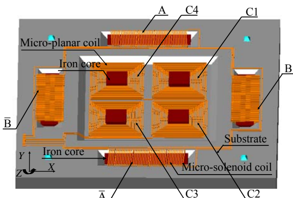
Figure 3 Tri-axis Micro-power Receiver
