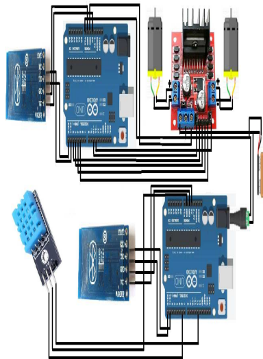
FIGURE 4: CIRCUIT DIAGRAM
