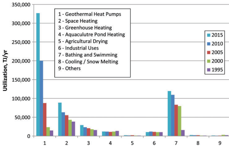
Figure 1.14. Comparison of worldwide direct-use geothermal energy in TJ year -1 from 1995, 2000, 2005, 2010 and 2015 (Lund and Boyd, 2016).
